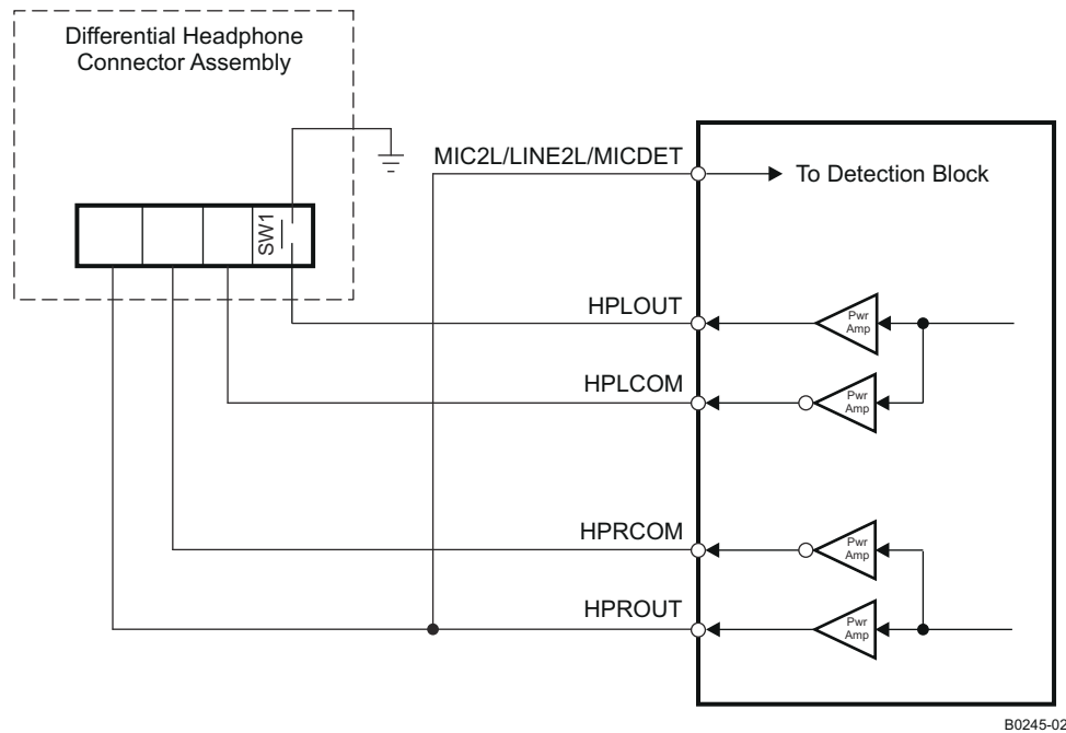
图 10-20. Configuration of Device for Jack Detection Using a Fully Differential Stereo Headphone Output Connection
