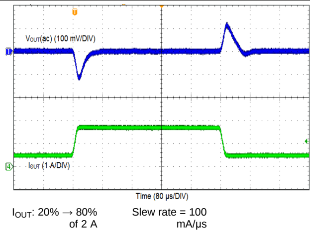
Figure 28. Load Transient
