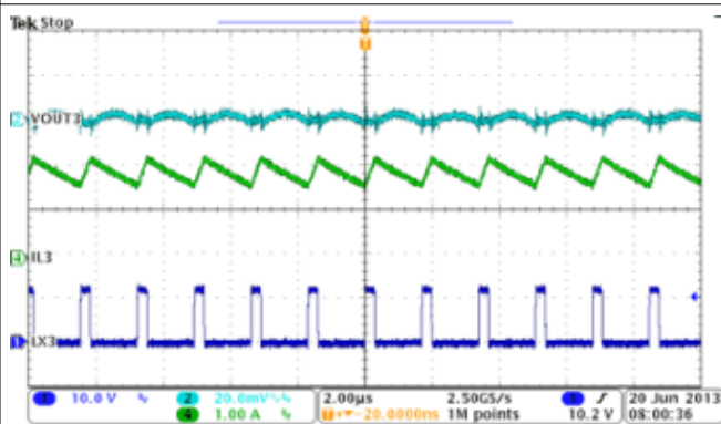
图 8-14. BUCK3, Steady State Operation with Full Load
