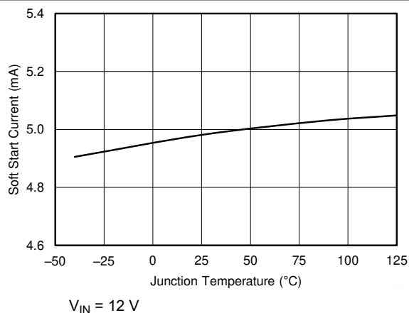
图 6-16. SS Pin Charge Current vs Temperature
