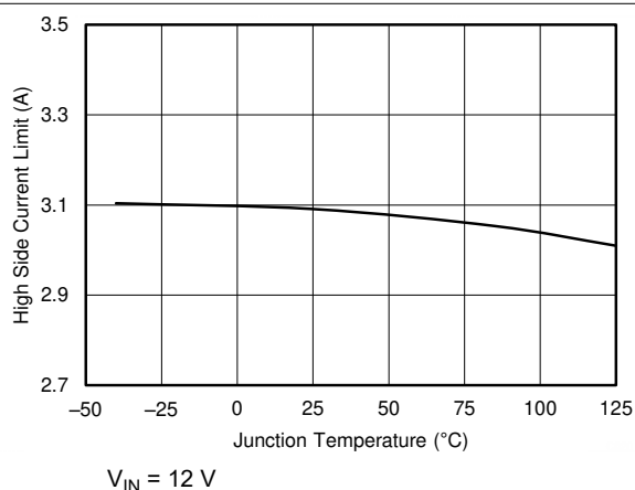
图 6-18. Buck2 High-Side Current Limit vs Temperature
