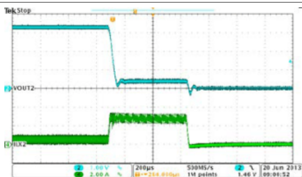
图 8-23. BUCK2, Overcurrent Protection
