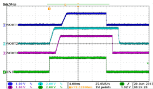
图 8-29. Automatic Power Sequencing, MODE=EN1= HIGH, EN2=LOW
