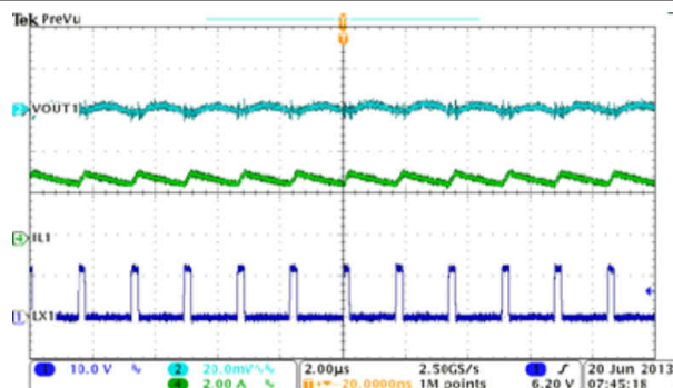
图 8-10. BUCK1, Steady State Operation with Full Load
