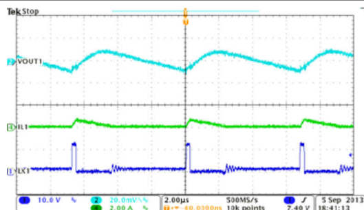
图 8-9. BUCK1, PSM Mode, Steady State Operation at Light Load
