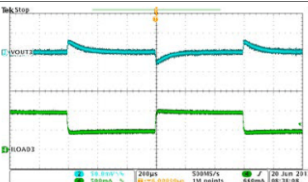
图 8-19. BUCK3, Load Transient, 0.5 A to 1.0 A SR = 0.25 A/µs
