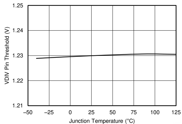
图 6-20. VDIV Pin Threshold vs Temperature
