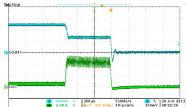
图 8-21. BUCK1, Overcurrent Protection
