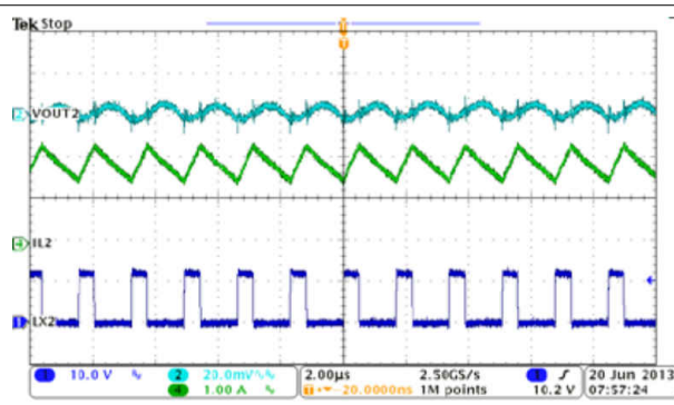
图 8-12. BUCK2, Steady State Operation with Full Load
