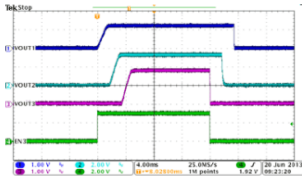
图 8-27. Automatic Power Sequencing, MODE=EN1=EN2=HIGH
