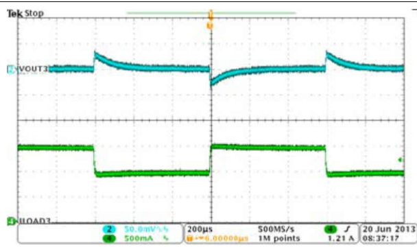
图 8-20. BUCK3, Load Transient, 1.0 A to 1.5 A SR = 0.25 A/µs
