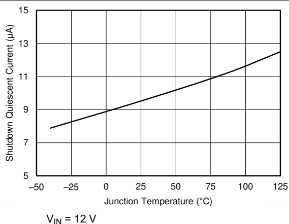
图 6-11. Shutdown Quiescent vs Temperature
