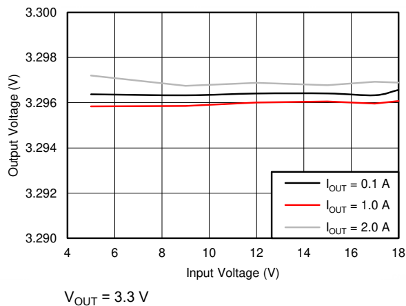
图 6-7. BUCK2, PSM MODE, LINE REGULATION
