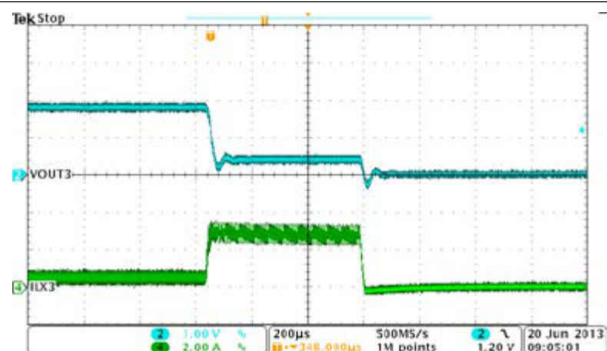
图 8-25. BUCK3, Overcurrent Protection
