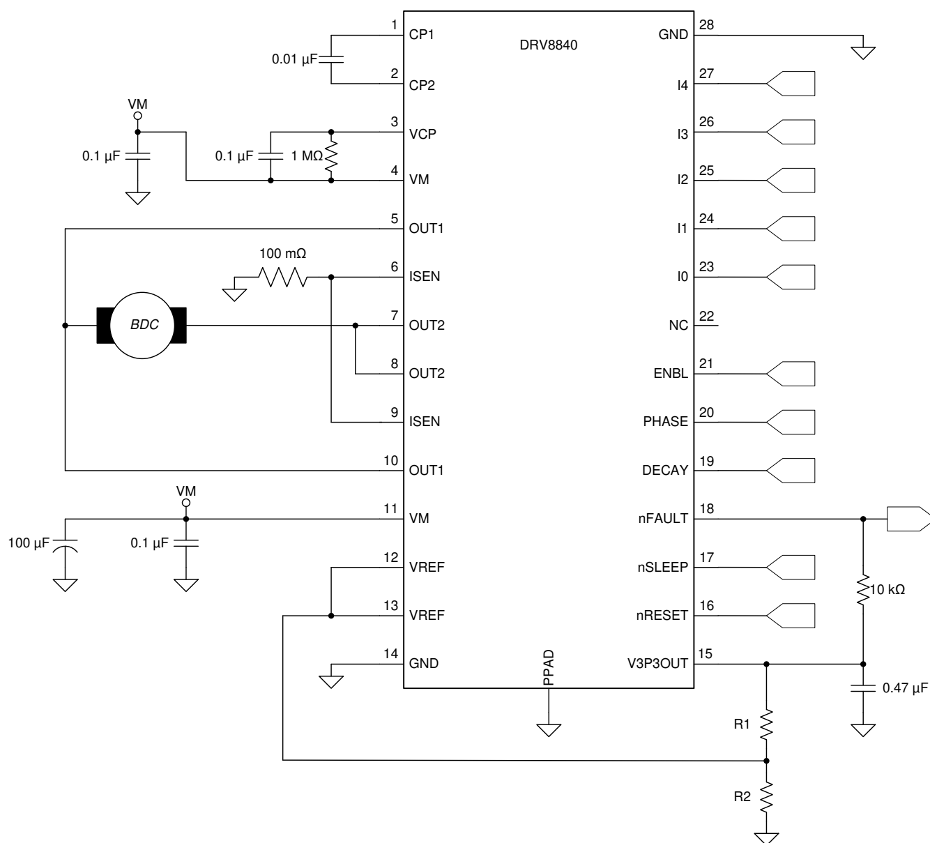
图 8-1. Typical Application Schematic
