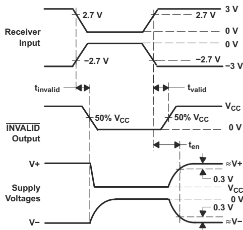
VOLTAGE WAVEFORMS
