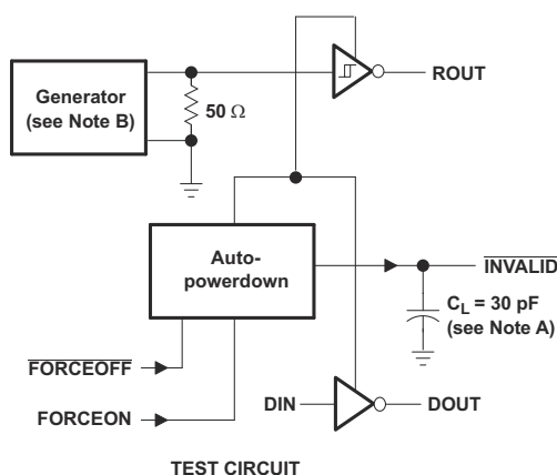
TEST CIRCUIT
