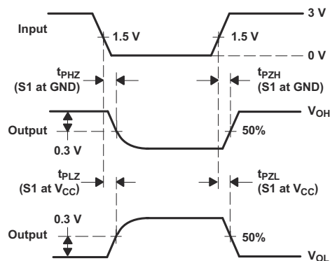
VOLTAGE WAVEFORMS
