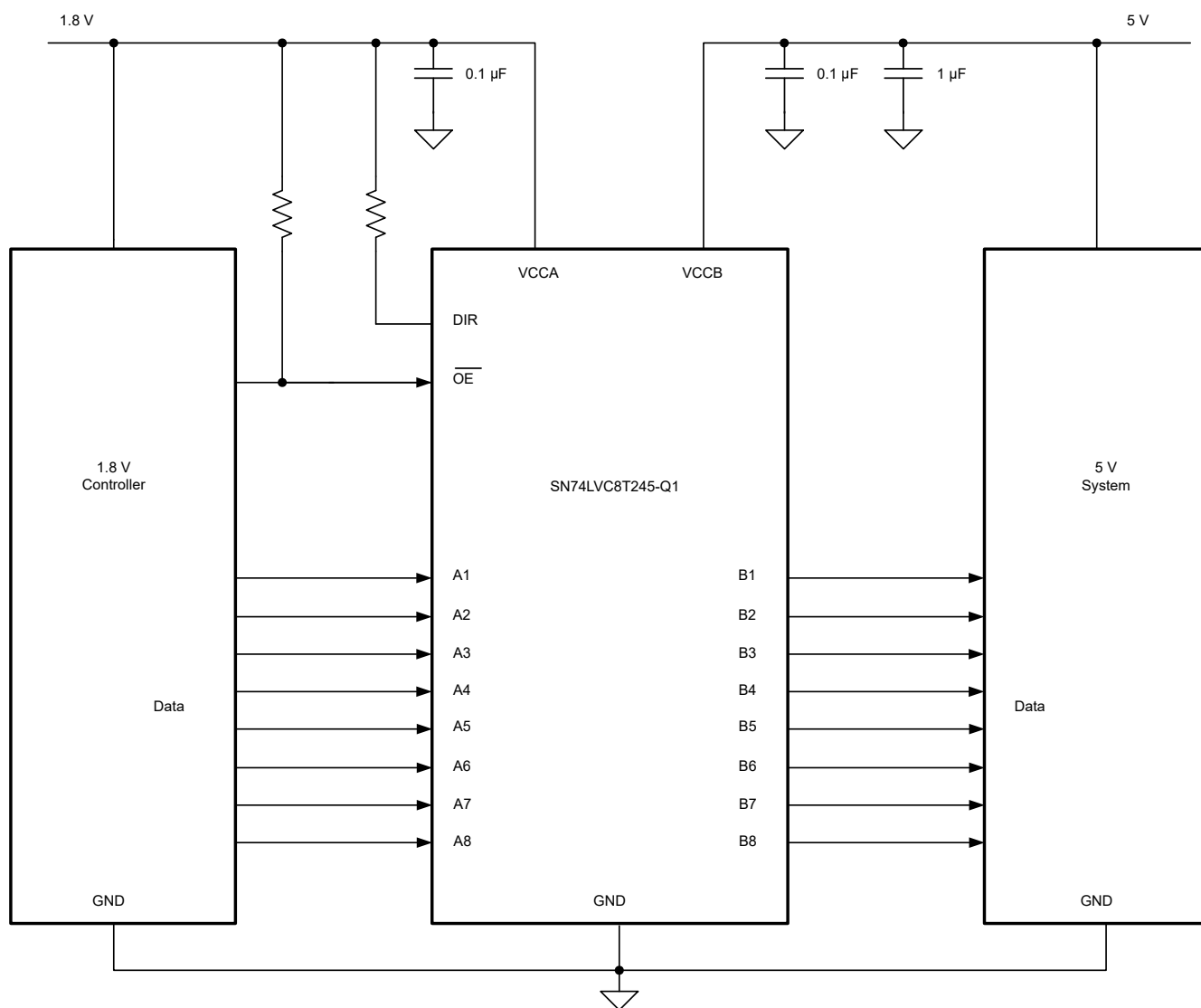
图 9-1. Typical Application Circuit
