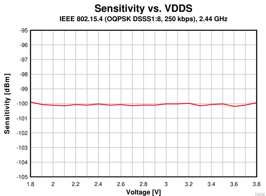
图 8-33. Sensitivity vs. Supply Voltage (VDDS) (250 kbps, 2.44 GHz)
