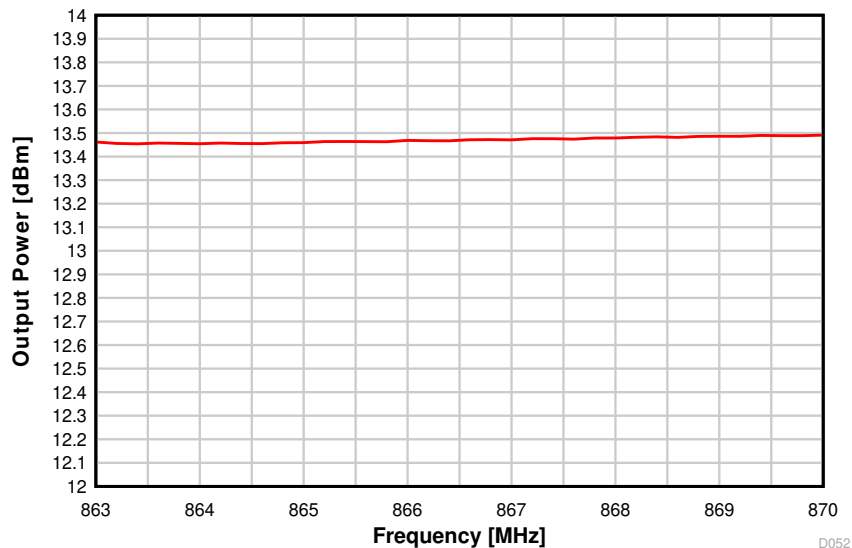
图 8-51. Output Power vs. Frequency (50 kbps, 868 MHz)
