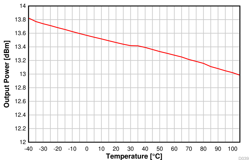
图 8-39. Output Power vs. Temperature (50 kbps, 868.3 MHz)
