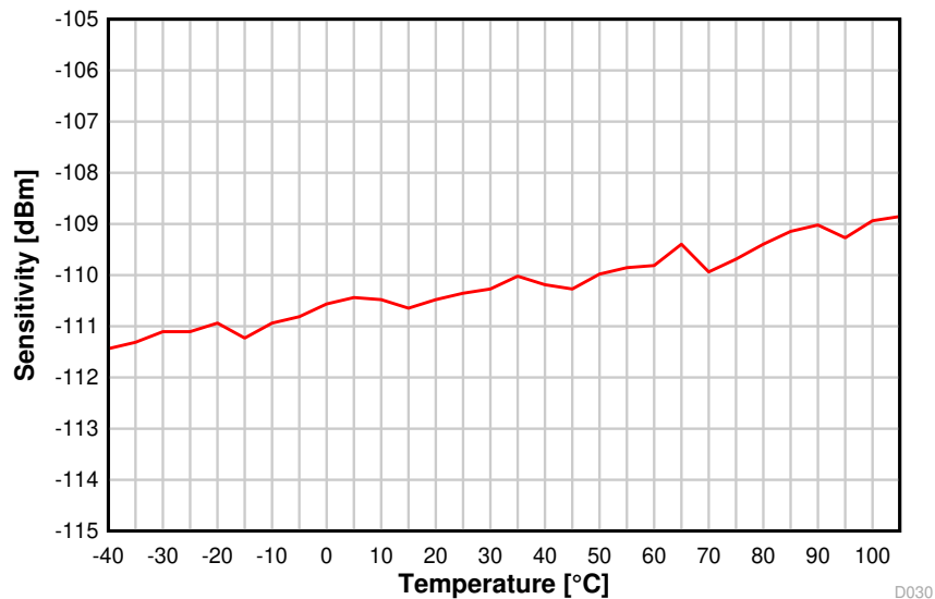
图 8-27. Sensitivity vs. Temperature (50 kbps, 868.3 MHz)
