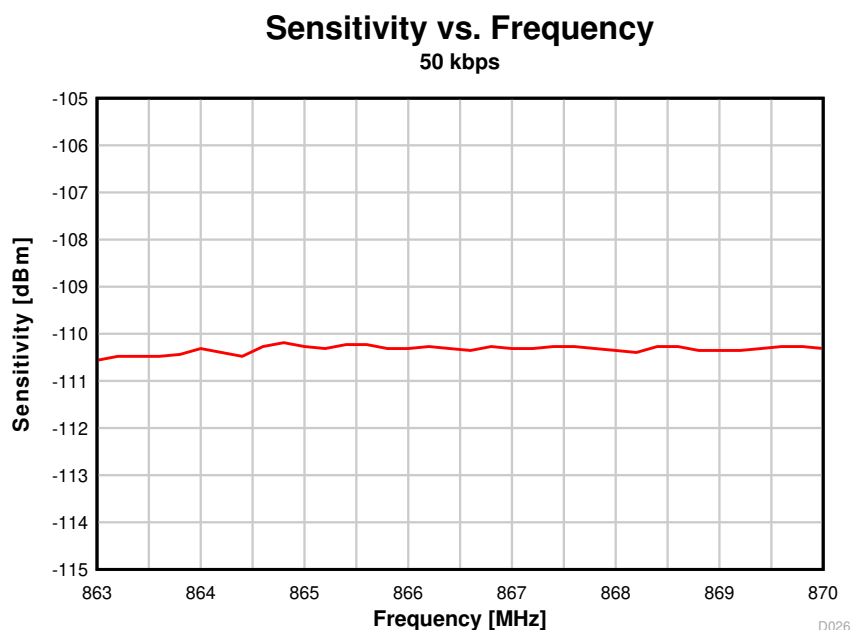
图 8-23. Sensitivity vs. Frequency (50 kbps, 868 MHz)
