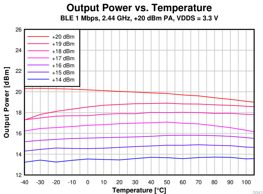
图 8-43. Output Power vs. Temperature (BLE 1 Mbps, 2.44 GHz, +20 dBm PA)
