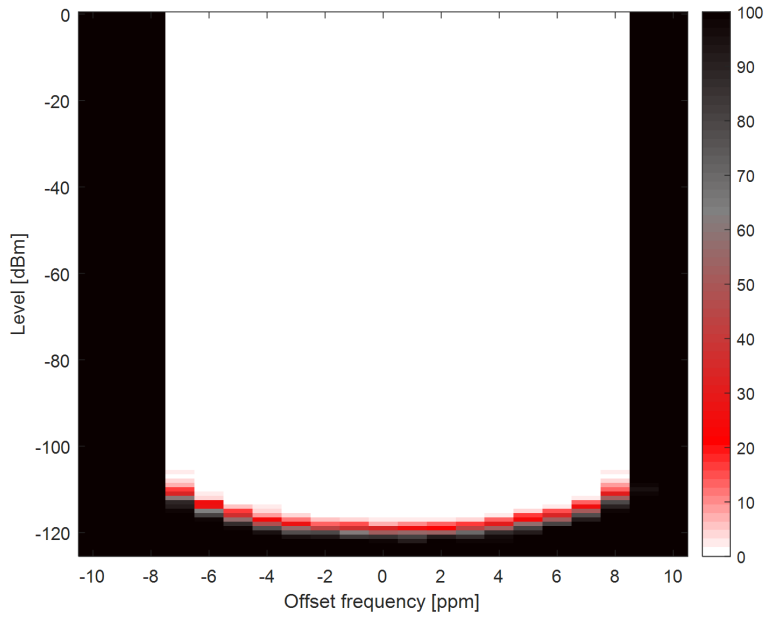
图 8-37. Narrowband, 4.8 kbps \pm 2 kHz deviation, 2-GFSK, 426.1 MHz, 10.1 kHz RX Bandwidth
