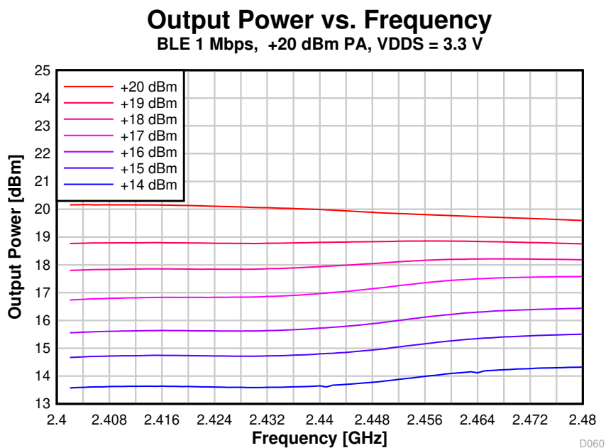
图 8-56. Output Power vs. Frequency (BLE 1 Mbps, 2.44 GHz, +20 dBm PA)
