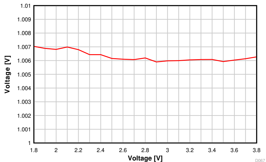
图 8-63. ADC Accuracy vs. Supply Voltage (VDD5)
