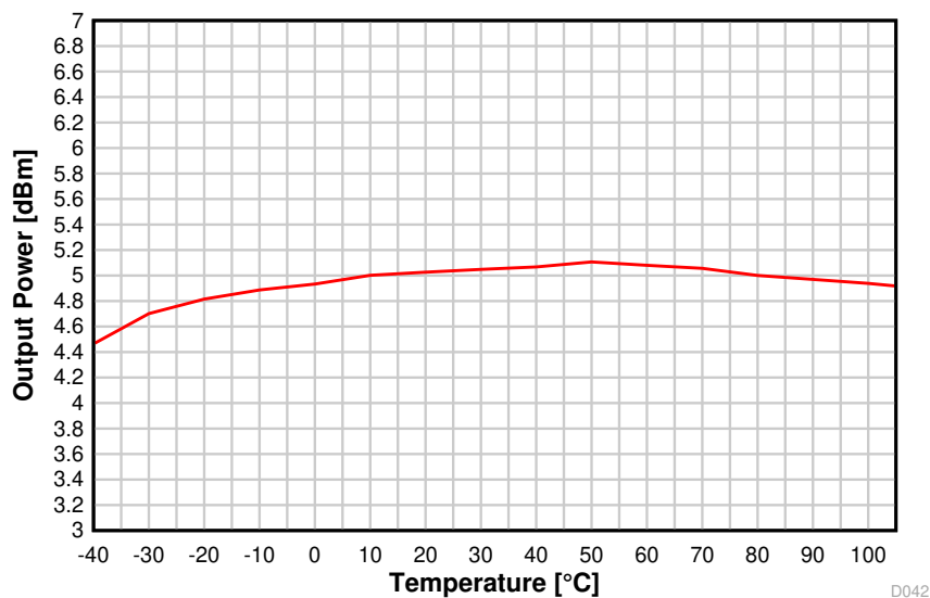
图 8-42. Output Power vs. Temperature (BLE 1 Mbps, 2.44 GHz, +5 dBm)
