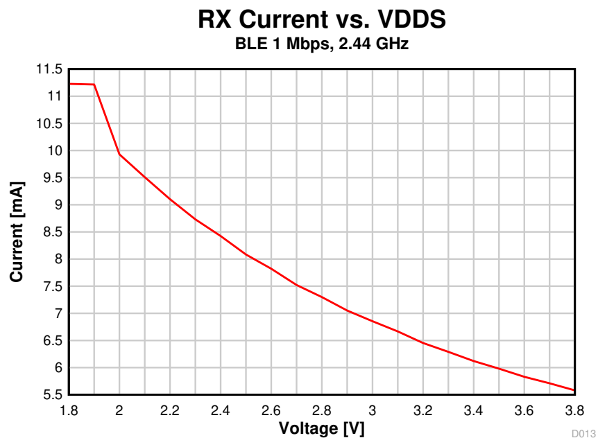
图 8-11. RX Current vs. Supply Voltage (VDDS) (BLE 1 Mbps, 2.44 GHz)
