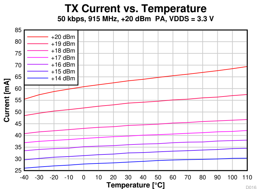
图 8-14. TX Current vs. Temperature (50 kbps, 915 MHz, VDD = 3.3 V)
