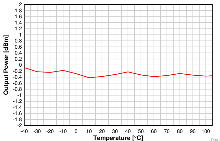
图 8-41. Output Power vs. Temperature (BLE 1 Mbps, 2.44 GHz)
