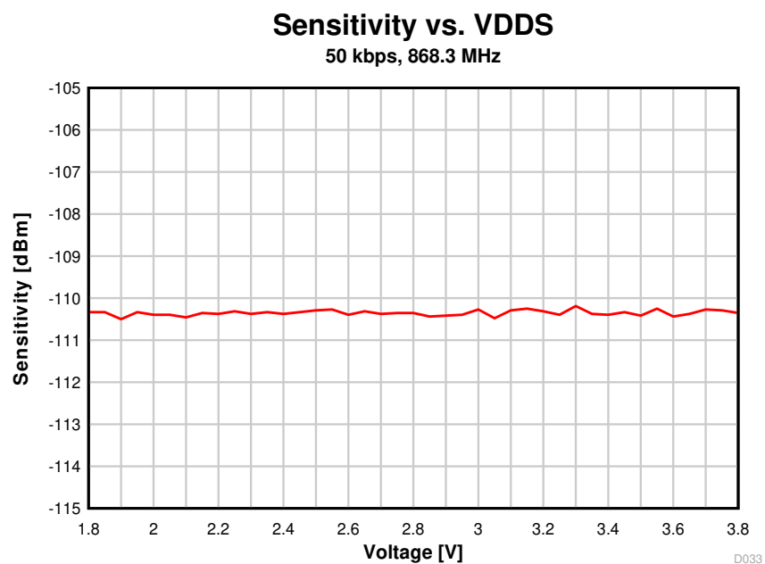
图 8-30. Sensitivity vs. Supply Voltage (VDDS) (50 kbps, 868.3 MHz)
