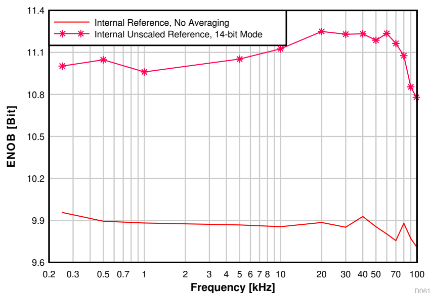
图 8-58. ENOB vs. Input Frequency
