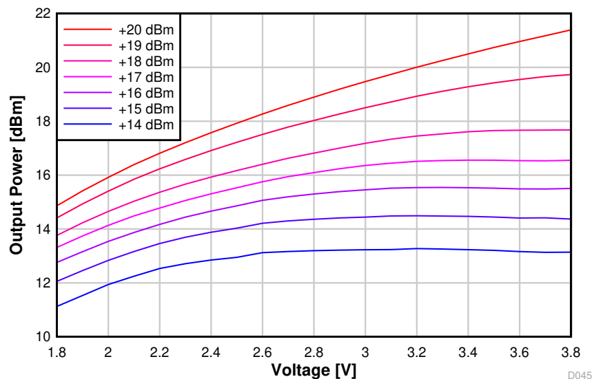
图 8-46. Output Power vs. Supply Voltage (VDDS) (50 kbps, 915 MHz)
