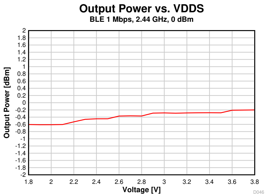
图 8-47. Output Power vs. Supply Voltage (VDD5) (BLE 1 Mbps, 2.44 GHz)
