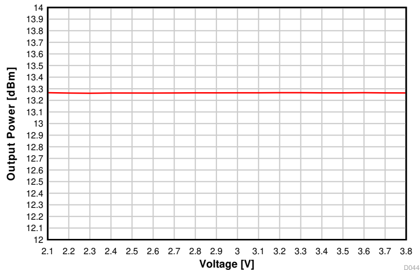
图 8-45. Output Power vs. Supply Voltage (VDDS) (50 kbps, 868.3 MHz)
