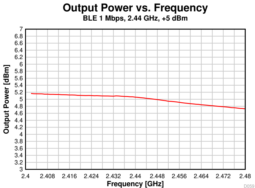
图 8-55. Output Power vs. Frequency (BLE 1 Mbps, 2.44 GHz, +5 dBm)
