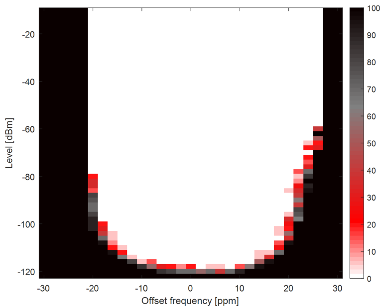
图 8-38. Narrowband, WMBUS N-MODE, 2.4 kbps, 169 MHz
