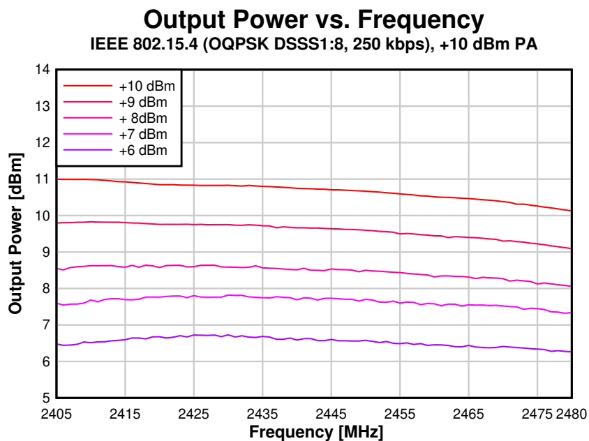
图 8-57. Output Power vs. Frequency (250 kbps, +10 dBm PA)
