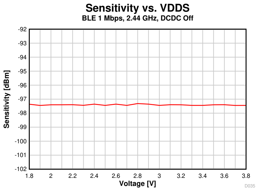
图 8-32. Sensitivity vs. Supply Voltage (VDDS) (BLE 1 Mbps, 2.44 GHz, DCDC Off)
