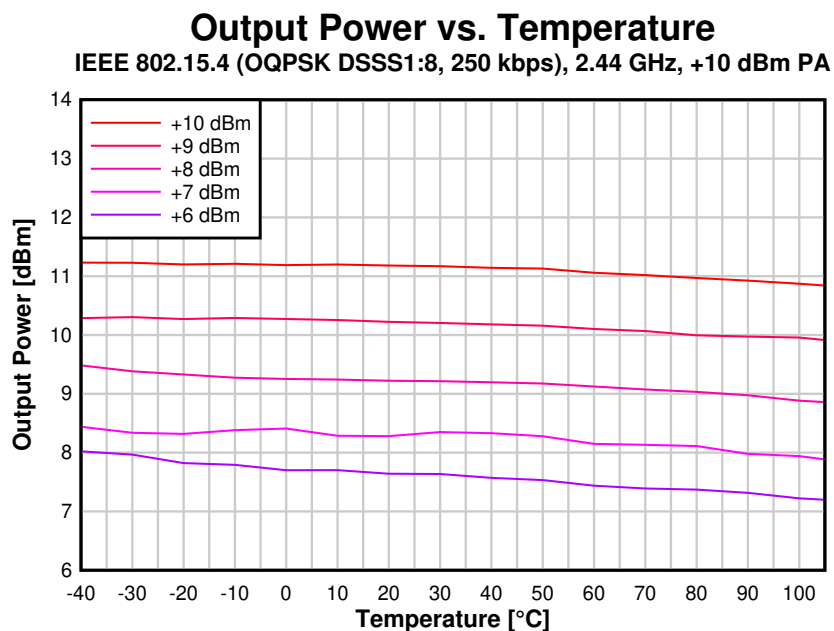
图 8-44. Output Power vs. Temperature (2.44 GHz, +10 dBm PA)
