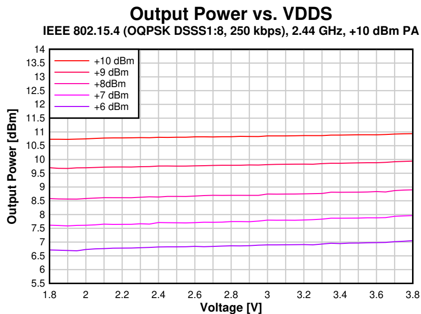
图 8-50. Output Power vs. Supply Voltage (VDDS) (2.44 GHz, +10 dBm PA)
