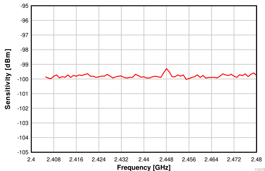
图 8-26. Sensitivity vs. Frequency (250 kbps, 2.44 GHz)
