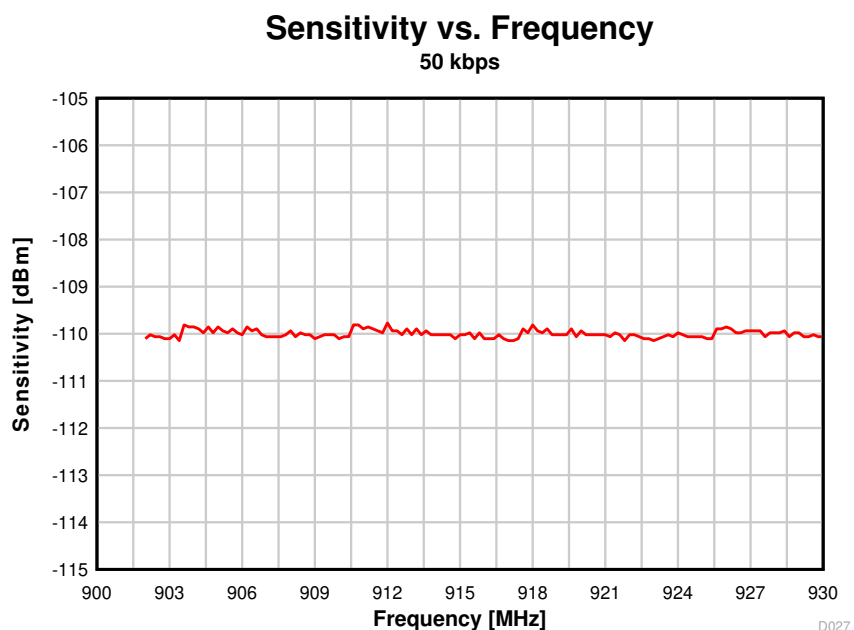
图 8-24. Sensitivity vs. Frequency (50 kbps, 915 MHz)
