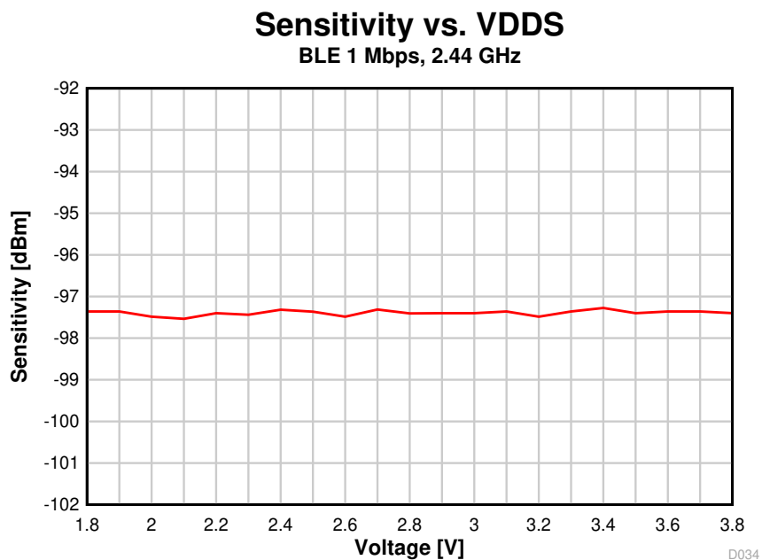
图 8-31. Sensitivity vs. Supply Voltage (VDDS) (BLE 1 Mbps, 2.44 GHz)
