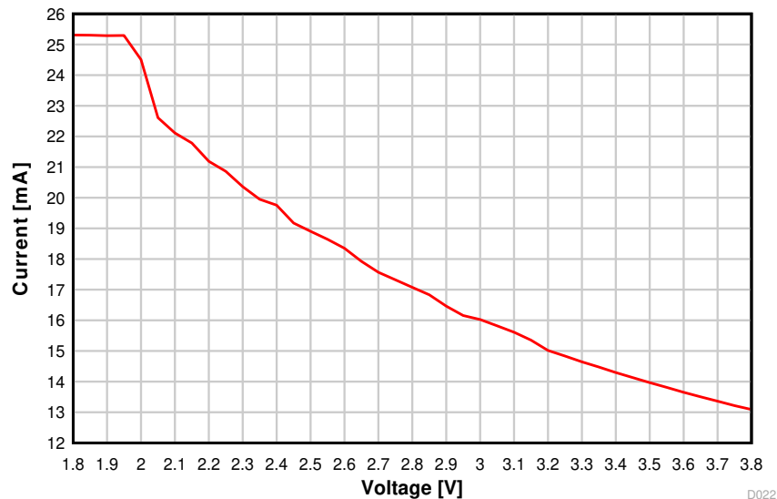
图 8-18. TX Current vs. Supply Voltage (VDDS) (50 kbps, 868.3 MHz)
