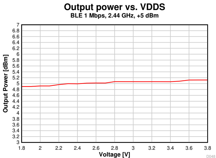
图 8-48. Output Power vs. Supply Voltage (VDD5) (BLE 1 Mbps, 2.44 GHz, +5 dBm)
