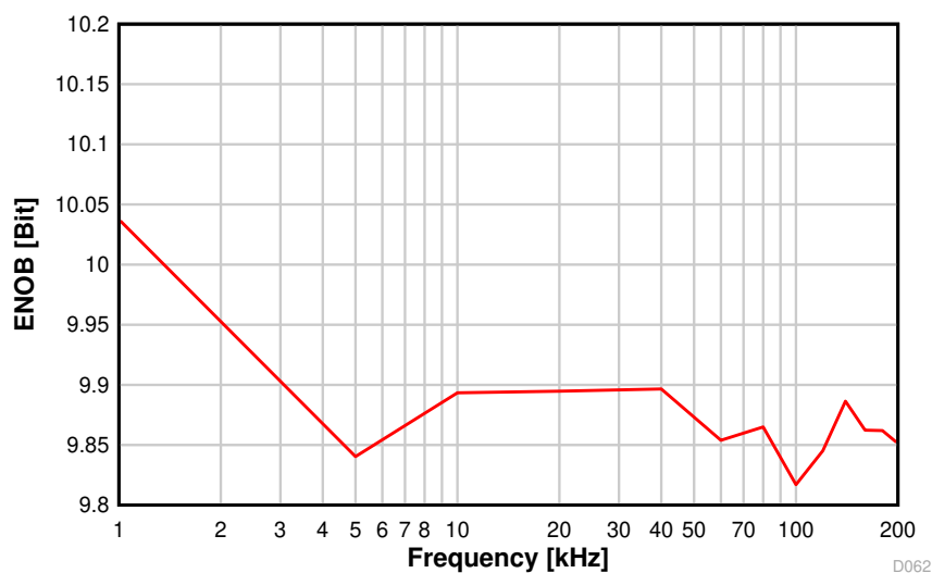
图 8-59. ENOB vs. Sampling Frequency
