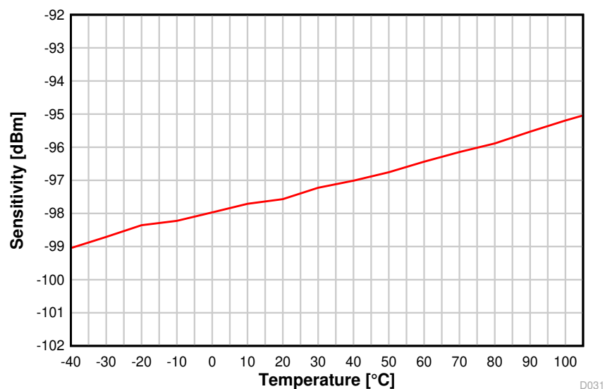
图 8-28. Sensitivity vs. Temperature (BLE 1 Mbps, 2.44 GHz)
