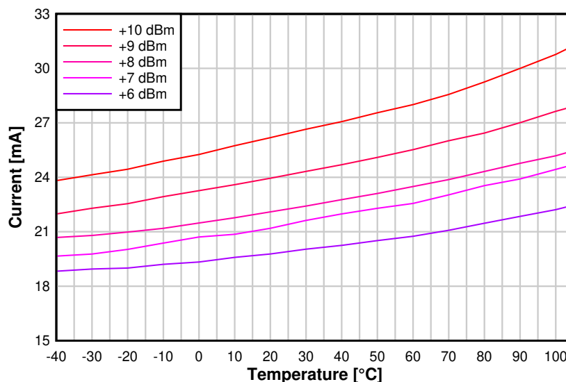
图 8-17. TX Current vs. Temperature (250 kbps, 2.44 GHz, +10 dBm PA)
