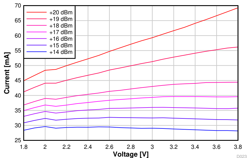
图 8-19. TX Current vs. Supply Voltage (VDDS) (50 kbps, 915 MHz)
