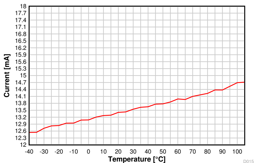
图 8-13. TX Current vs. Temperature (50 kbps, 868.3 MHz, VDD = 3.6 V)
