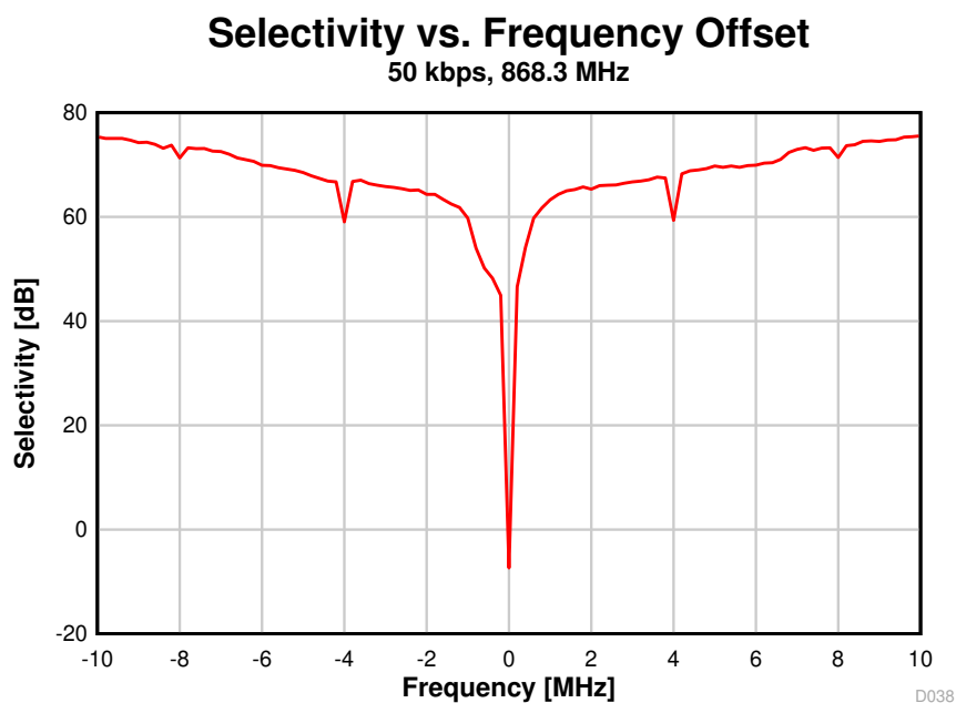
图 8-34. Selectivity vs. Frequency Offset (50 kbps, 868.3 MHz)
