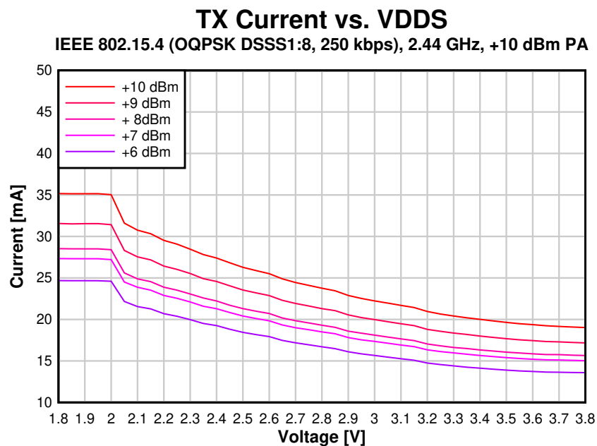
图 8-22. TX Current vs. Supply Voltage (VDDS) (250 kbps, 2.44 GHz, +10 dBm PA)
