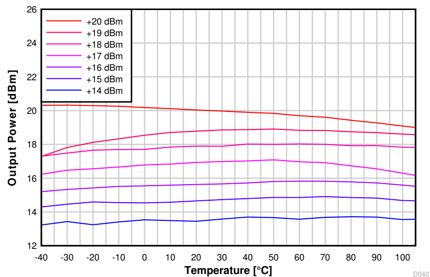
图 8-40. Output Power vs. Temperature (50 kbps, 915 MHz)
