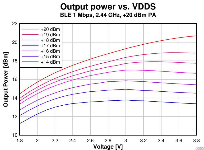
图 8-49. Output Power vs. Supply Voltage (VDDS) (BLE 1 Mbps, 2.44 GHz, +20 dBm PA)
