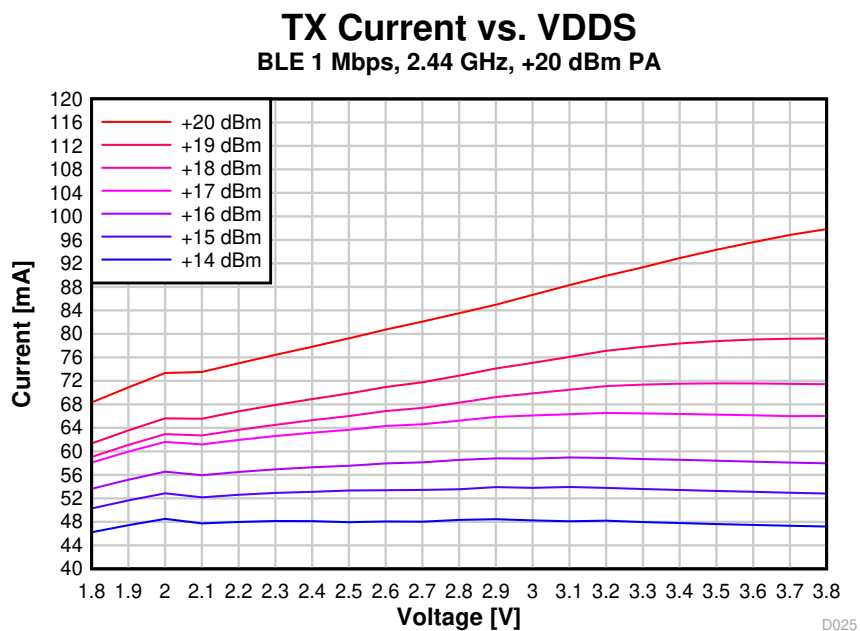
图 8-21. TX Current vs. Supply Voltage (VDD5) (BLE 1 Mbps, 2.44 GHz, +20 dBm PA)
