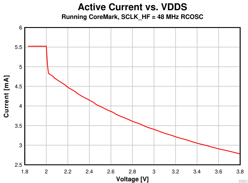
图 8-4. Active Mode (MCU) Current vs. Supply Voltage (VDDS)
