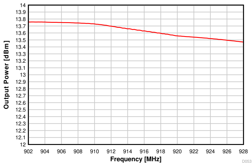
图 8-52. Output Power vs. Frequency (50 kbps, 915 MHz)
