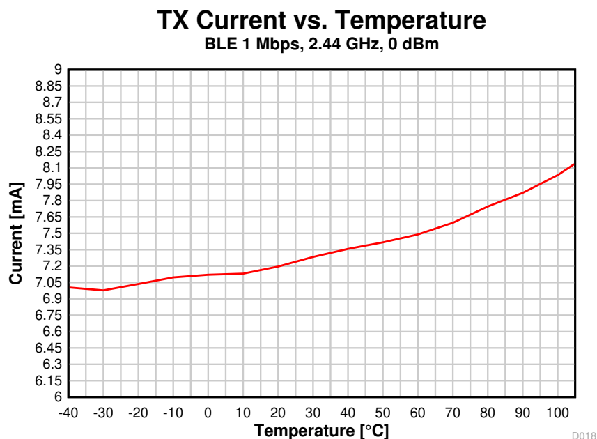
图 8-15. TX Current vs. Temperature (BLE 1 Mbps, 2.44 GHz)
