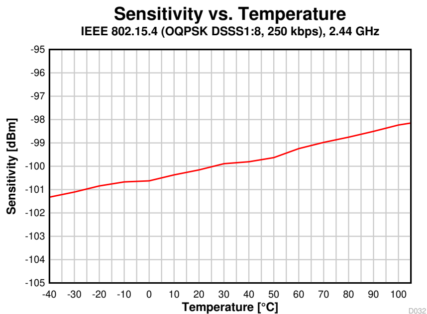
图 8-29. Sensitivity vs. Temperature (250 kbps, 2.44 GHz)
