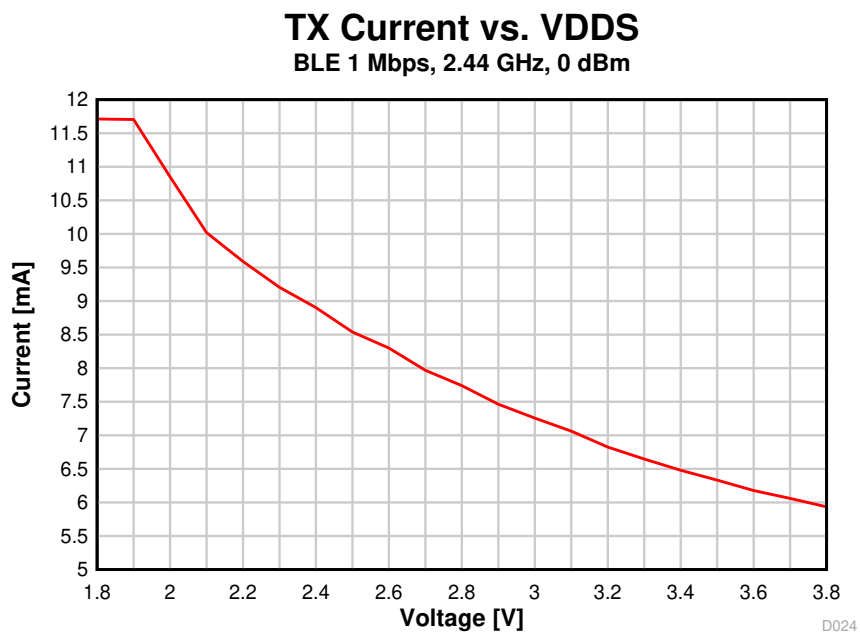
图 8-20. TX Current vs. Supply Voltage (VDD5) (BLE 1 Mbps, 2.44 GHz)
