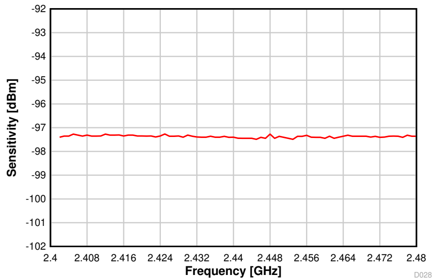
图 8-25. Sensitivity vs. Frequency (BLE 1 Mbps, 2.44 GHz)
