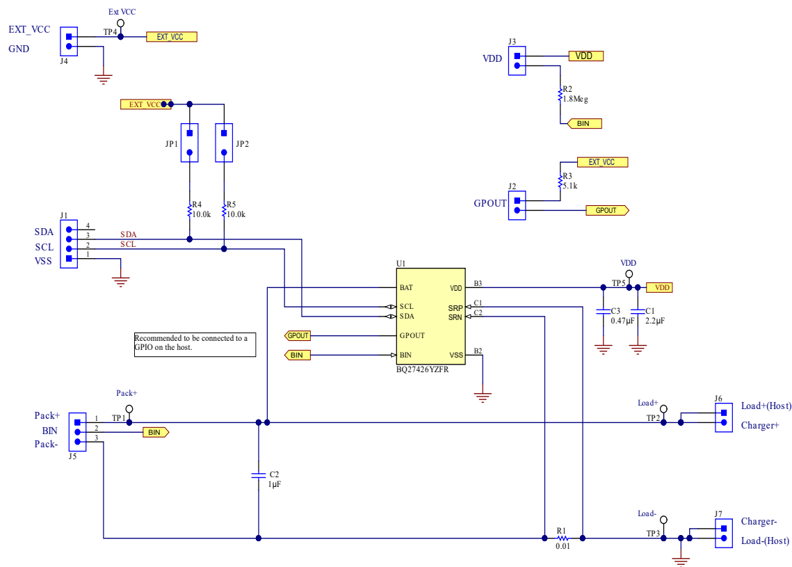
图 8-2. Typical Application with Low-Side Current Sense Resistor
