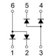
BAT54ADW
