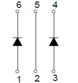
BAT54JW
