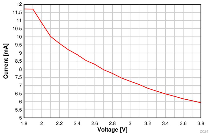
图 8-16. TX Current vs. Supply Voltage (VDDS) (BLE 1 Mbps, 2.44 GHz)
