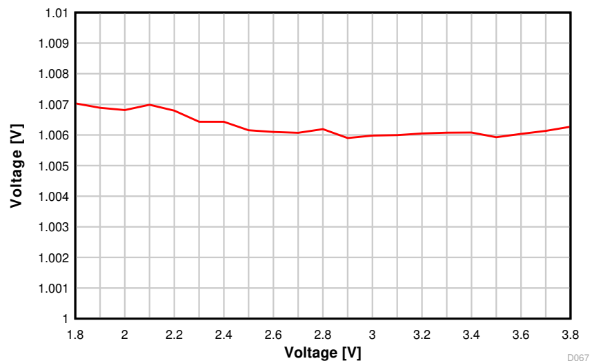
图 8-48. ADC Accuracy vs. Supply Voltage (VDDS)
