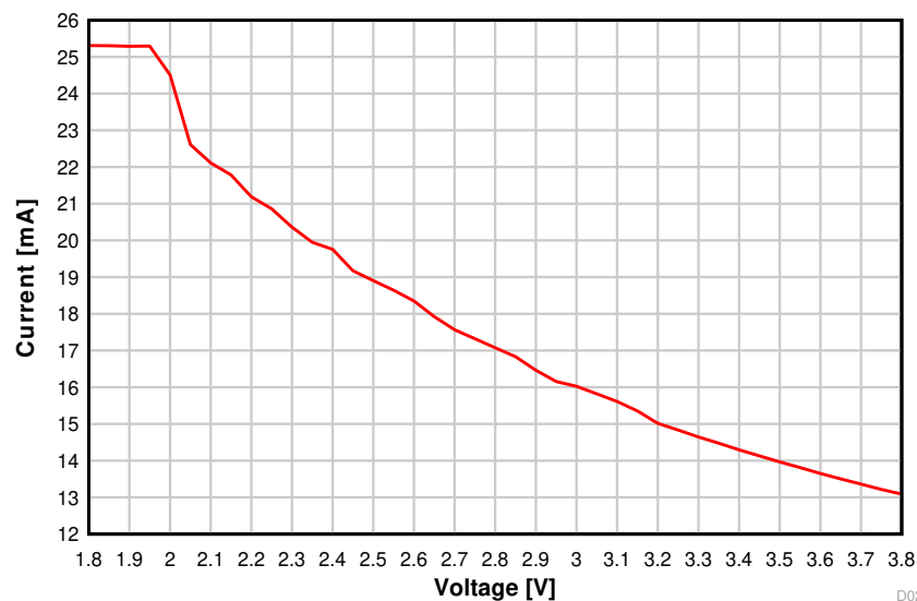
图 8-15. TX Current vs. Supply Voltage (VDDS) (50 kbps, 868.3 MHz)
