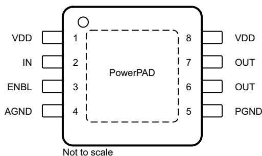
图 6-2. DGN Package 8-Pin MSOP with PowerPAD Top View
