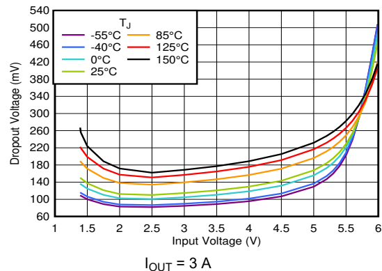
图 6-66. Dropout Voltage vs V_{IN} Without Bias
