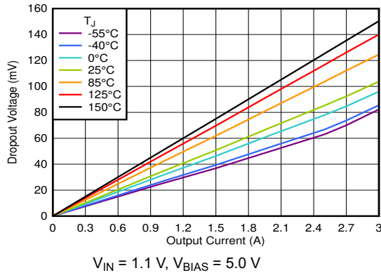
图 6-69. Dropout Voltage vs I_{OUT} With Bias
