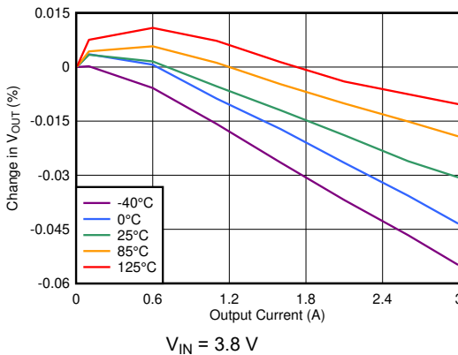
图 6-27. Load Regulation vs I_{OUT} (3.3-V Output)
