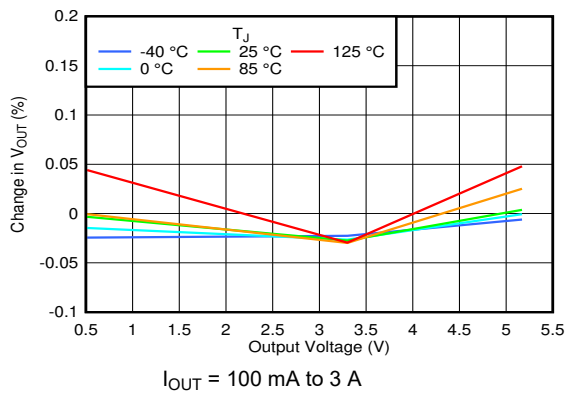
图 6-71. Load Regulation vs V_{OUT}
