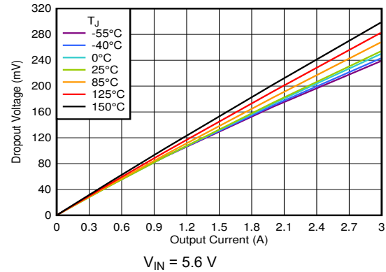
图 6-70. Dropout Voltage vs I_{OUT} (High V_{IN} )
