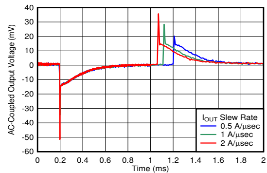
图 6-62. Load Transient vs Time and V_{OUT} Without Bias
