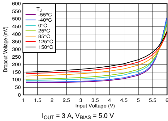
图 6-67. Dropout Voltage vs V_{IN} With Bias
