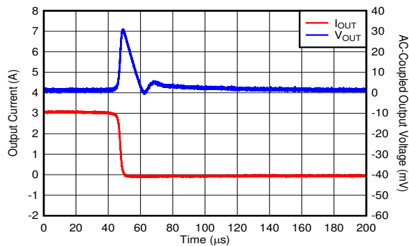
图 6-61. Load Transient vs Time and V_{OUT} With Bias
