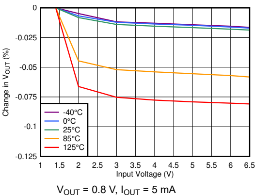
图 6-29. Line Regulation vs V_{IN}
