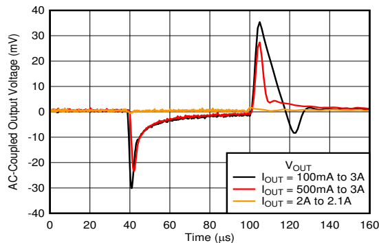
图 6-63. Load Transient vs Time and V_{OUT} Without Bias
