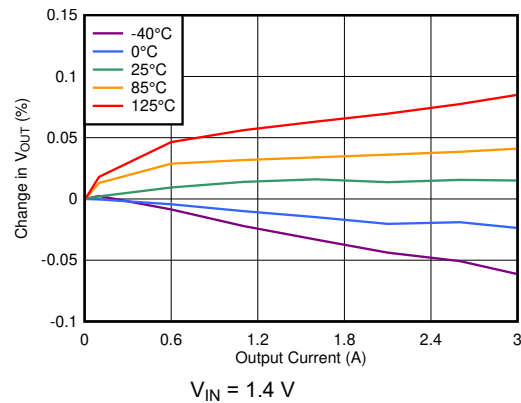
图 6-26. Load Regulation vs I_{OUT}
