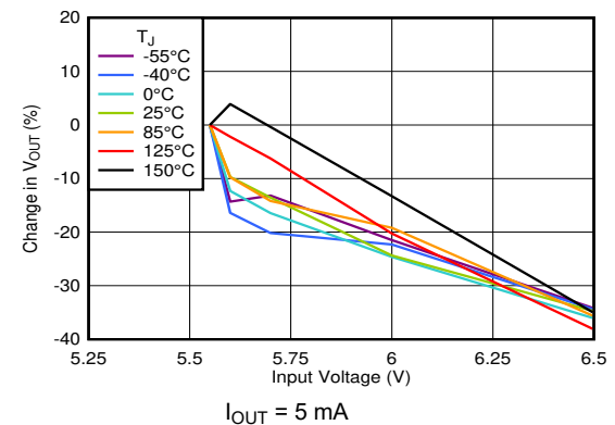
图 6-77. Line Regulation vs V_{IN} (5.15-V Output)
