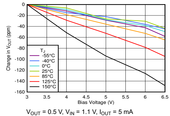
图 6-76. Line Regulation With Bias
