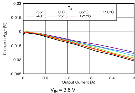
图 6-73. Load Regulation vs I_{OUT} (3.3-V Output)
