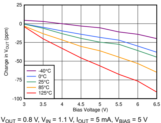
图 6-30. Line Regulation With Bias
