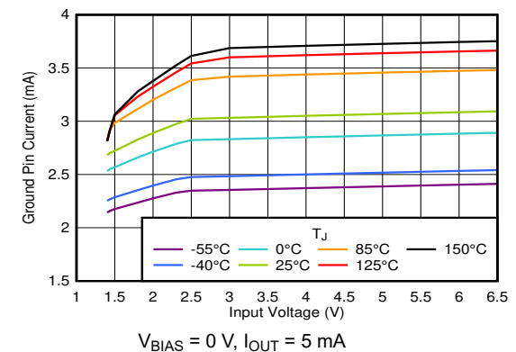
图 6-78. Ground Pin Current vs V_{IN}
