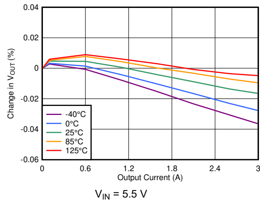
图 6-28. Load Regulation vs I_{OUT} (5-V Output)
