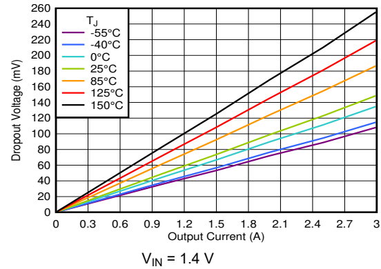
图 6-68. Dropout Voltage vs I_{OUT} Without Bias
