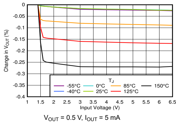
图 6-75. Line Regulation vs V_{IN}
