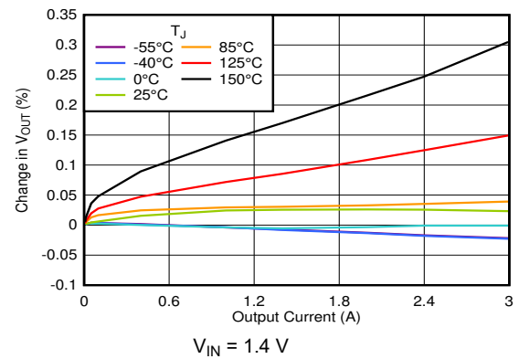
图 6-72. Load Regulation vs I_{OUT}
