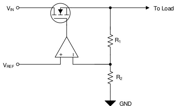
图 7-3. Simplified Regulation Circuit
