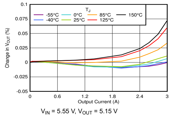
图 6-74. Load Regulation vs I_{OUT} (5-V Output)
