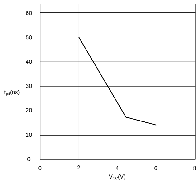
Figure 7. SN74HC595B t_{pd} vs. V_{CC}
