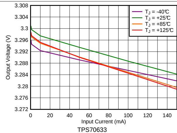
Figure 4. 3.3-V Load Regulation vs I_{\text{OUT}} and Temperature
