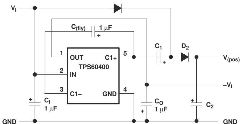
图 9-7. TPS60400 as Doubler/Inverter
