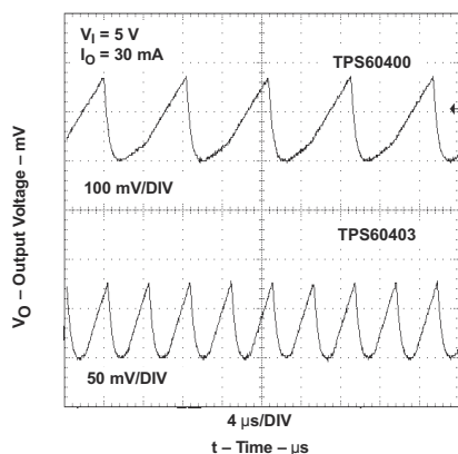
图 9-2. Output Voltage vs Time for TPS60400 and TPS60401
