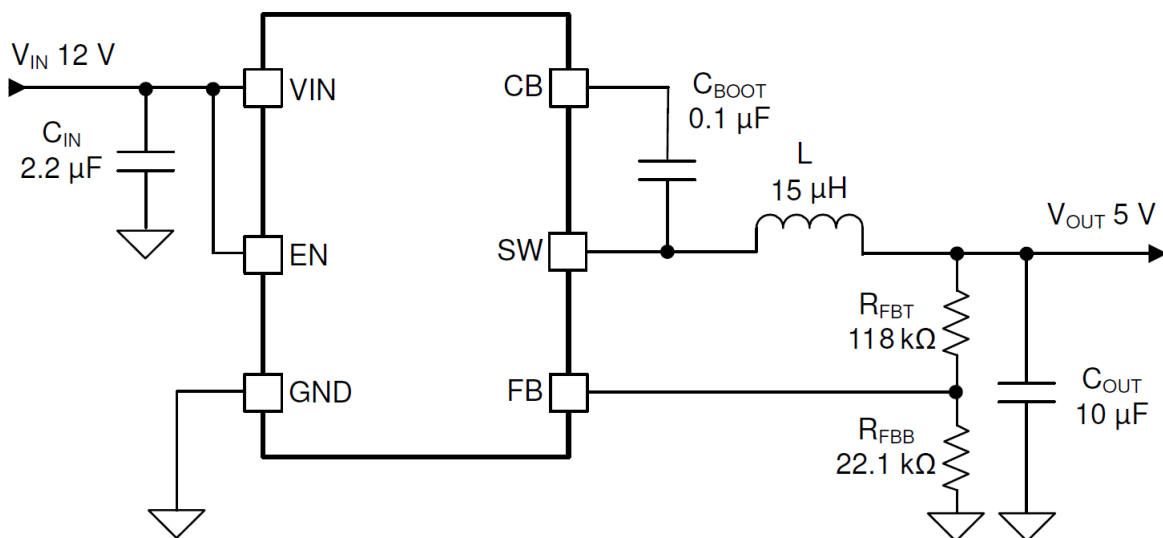
图 8-1. Application Circuit
