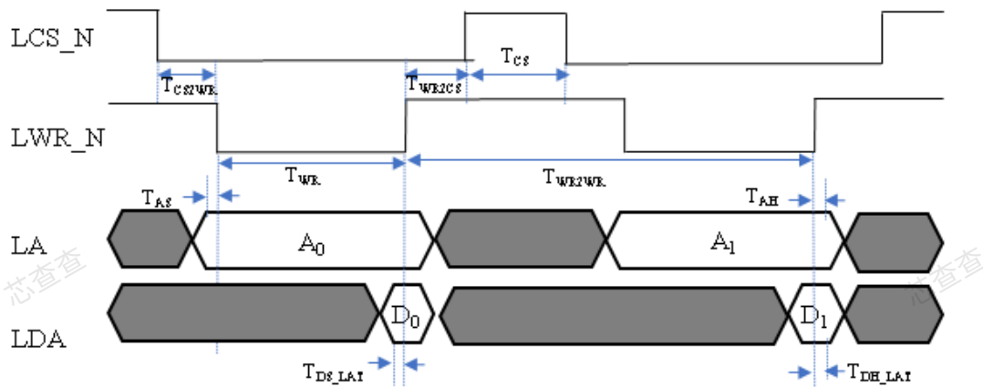
Figure 4-29: Function Local Bus Write Access (Late Sample = 1)
