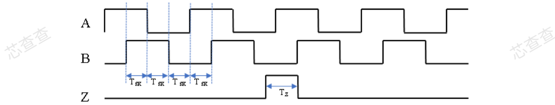
Figure 4-34: ABZ Timing Diagram
