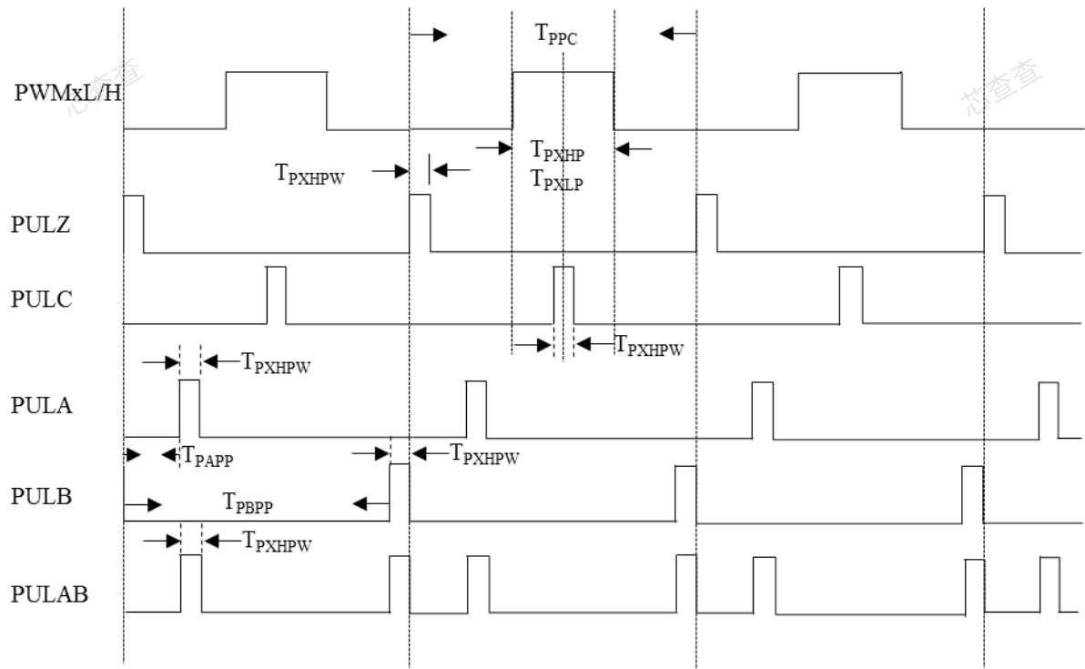
Figure 4-30: PWMx Timing
