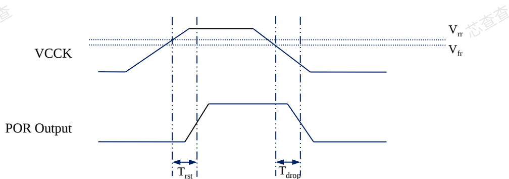
Figure 4-1: Power On Reset (POR) Timing Diagram
