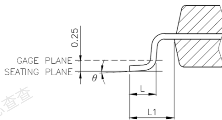
THERMALLY ENHANCED DIMENSIONS(SHOWN IN MM)
