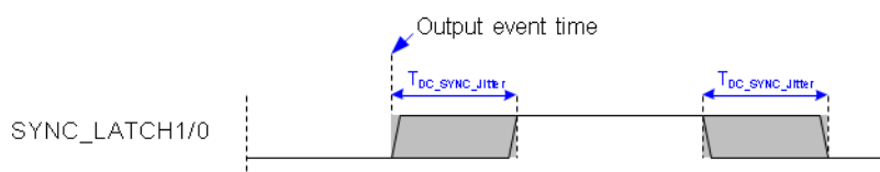
Figure 4-11: SYNC timing
