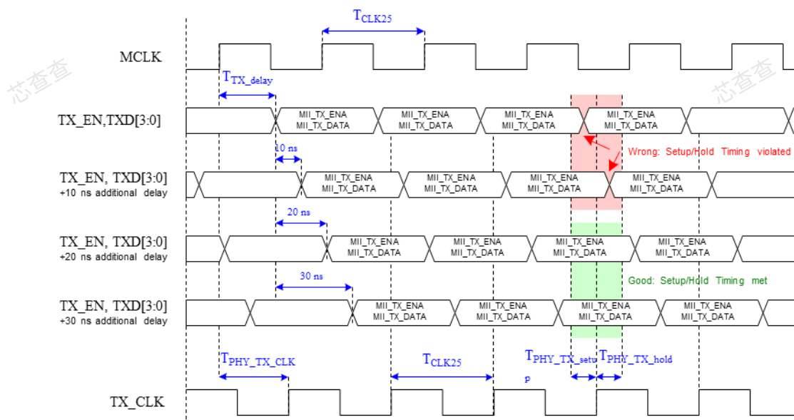
Figure 4-6: Port 2 MII TX Timing Diagram
