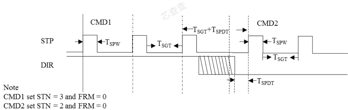
Figure 4-33: One Shot with multi Step Timing Diagram
