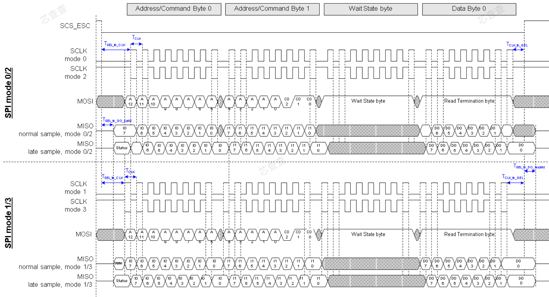
Figure 4-17: PDI SPI Slave read access (2 byte addressing, 1 byte read data) with Wait State byte
