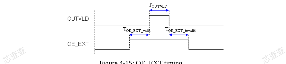
Figure 4-15: OE_EXT timing
