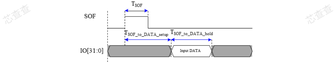
Figure 4-12: Digital Input: Input data sampled at SOF, IO can be read in the same frame
