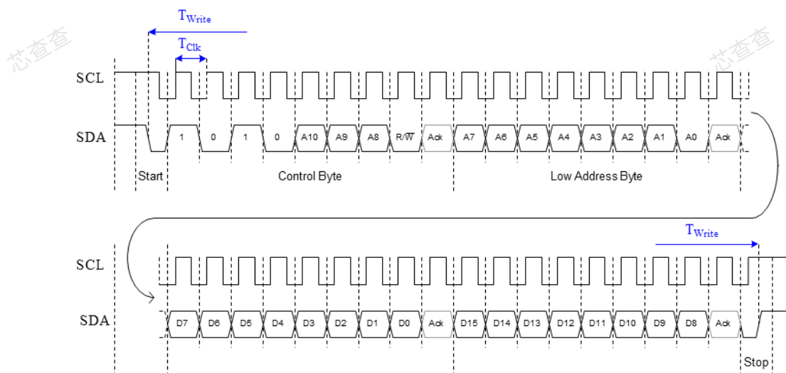
Figure 4-3: Write access (1 address byte, up to 16 Kbit EEPROMs)
