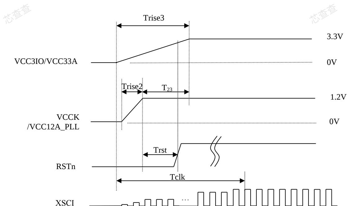
Figure 4-2: Power-up Sequence Timing Diagram
