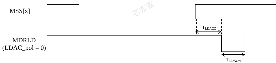
Figure 4-42: SPI MDRLD Trigger LDAC Gap and Width Timing
