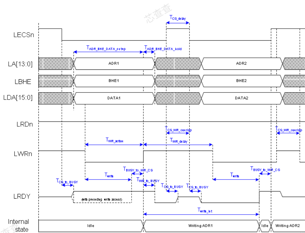
Figure 4-24: PDI Local Bus Write access (write after rising edge nWR, without preceding write access)
