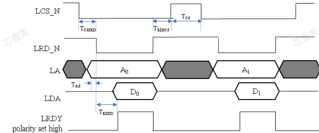
Figure 4-27: Function Local Bus Signal Read Access
