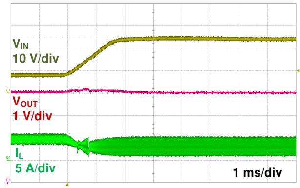
图 8-5. Line Transient Response (8 V - 24 V, I_{OUT} = 2 A)
