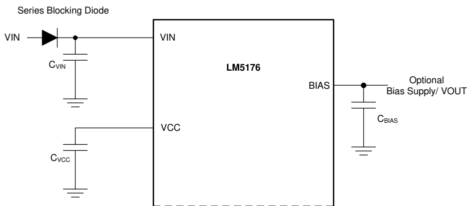
图 7-1. VCC Regulator and Optional BIAS
