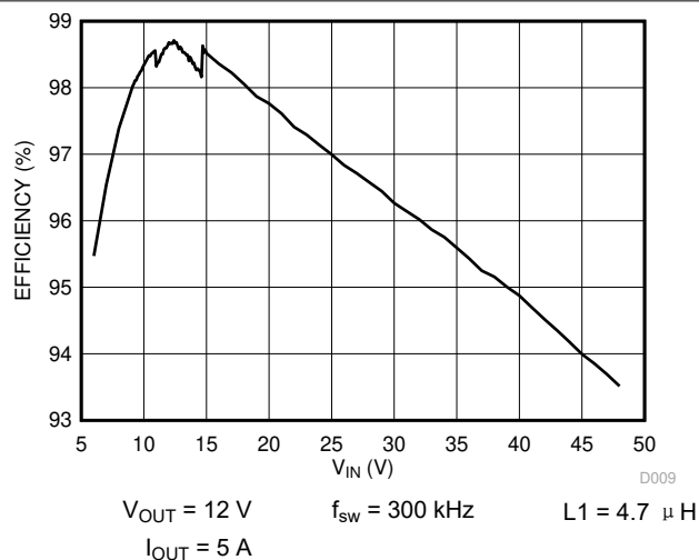
图 6-1. Efficiency vs V_{IN}
