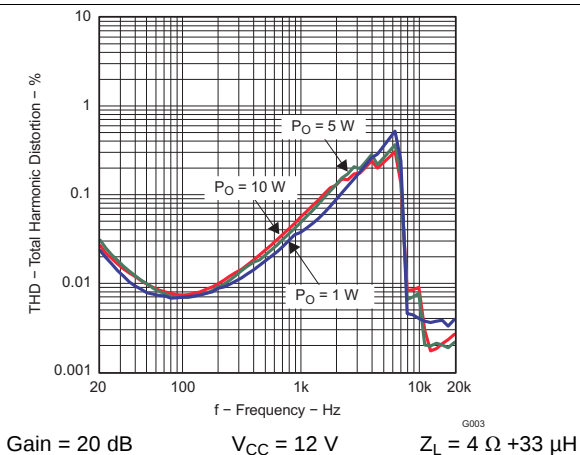
Figure 3. Total Harmonic Distortion vs Frequency
