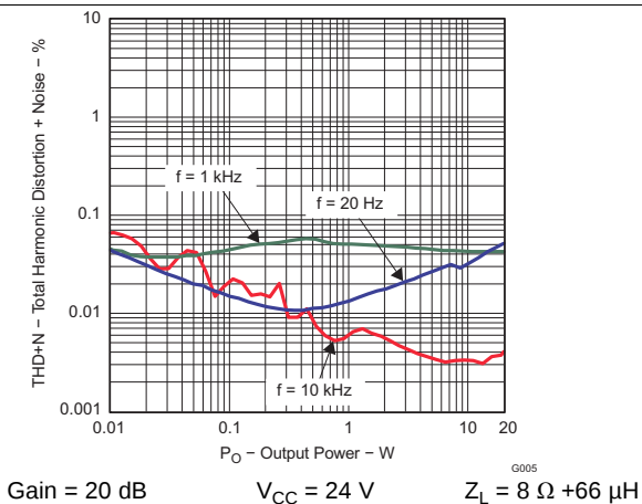
Figure 5. Total Harmonic Distortion + Noise vs Output Power
