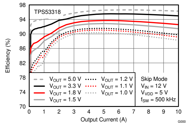
图 7-27. Efficiency vs Output Current
