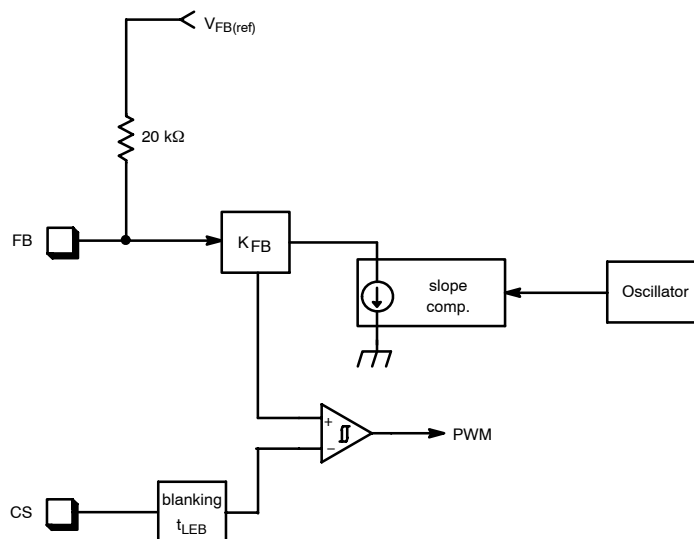
In order to allow the NCP1236 to operate in CCM with a duty cycle above 50 %, a fixed slope compensation is internally applied to the current-mode control. The slope
