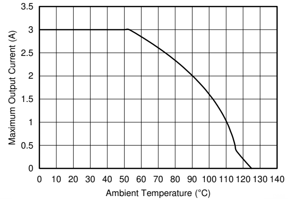
图 8-4. Maximum Output Current versus Ambient Temperature
