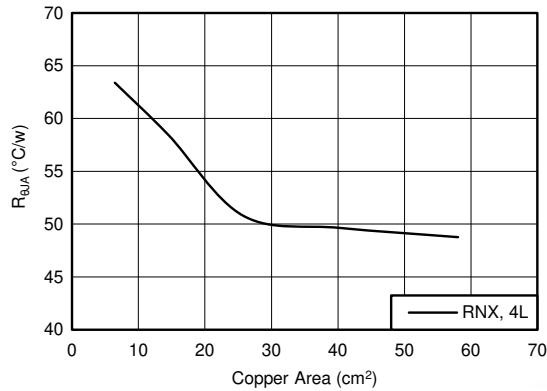
图 8-3. R_{\theta JA} versus Copper Board Area for the VQFN (RNX) Package
