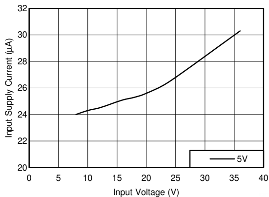
图 8-12. Input Supply Current
