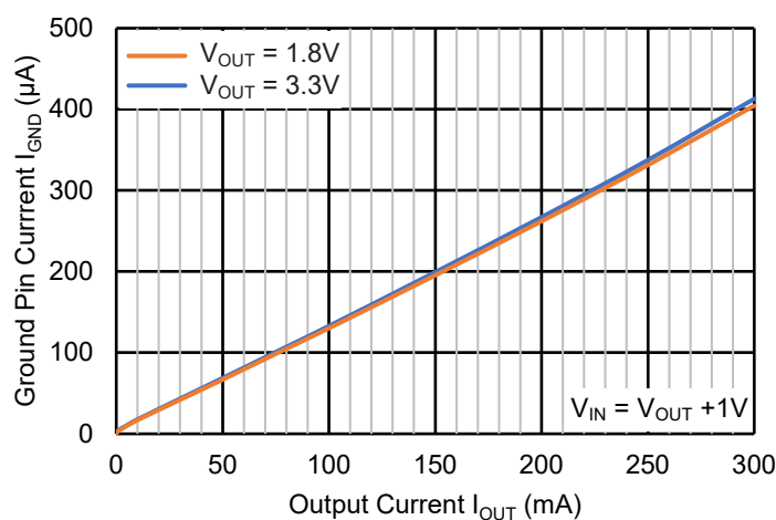
Ground Pin Current
