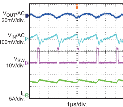
Input/Output Voltage Ripple I_{OUT} = 6A
