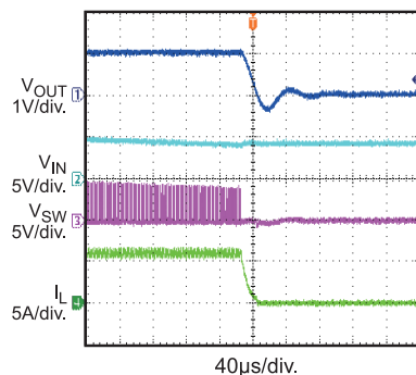
Shutdown Through VIN I_{OUT} = 6A
