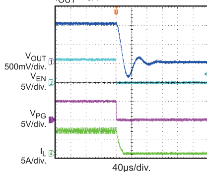
Power Good Through EN Shutdown I_{OUT} = 6A
