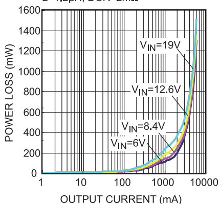
Power Loss
