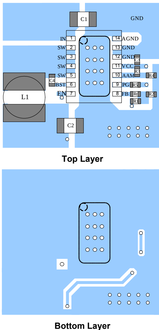
Figure 7—PCB Layout
