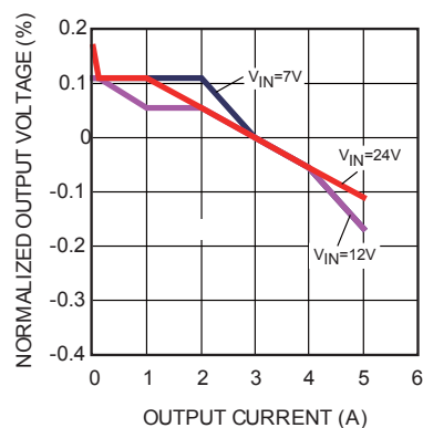
Load Regulation
