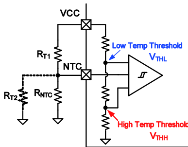
Figure 8: NTC Function Block
