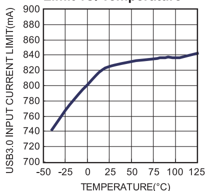
USB3.0 Input Current Limit vs. Temperature
