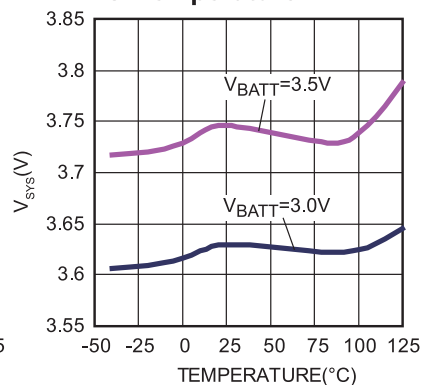
System Voltage Regulation vs. Temperature
