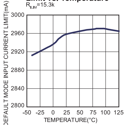
Program Mode Input Current Limit vs. Temperature R_{ILIM} = 15.3k
