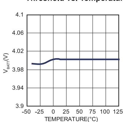
Battery Auto-recharge Threshold vs. Temperature
