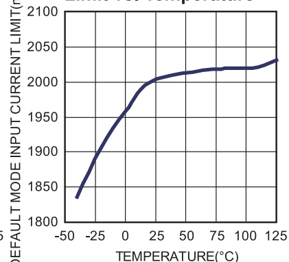
Default Mode Input Current Limit vs. Temperature
