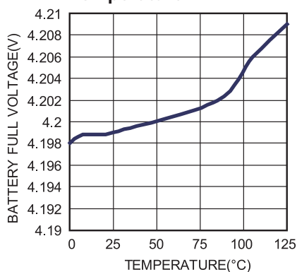
Battery Regulation vs. Temperature
