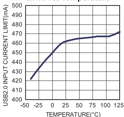
USB2.0 Input Current Limit vs. Temperature
