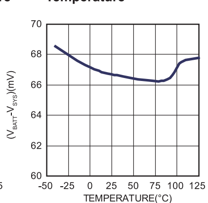
Ideal Diode Regulation vs. Temperature
