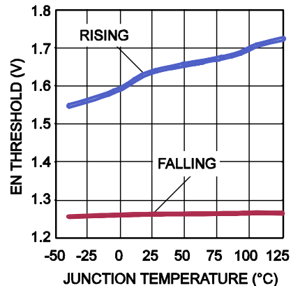
EN Threshold vs. Junction Temperature
