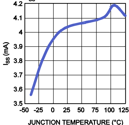
I_{SS} vs. Junction Temperature
