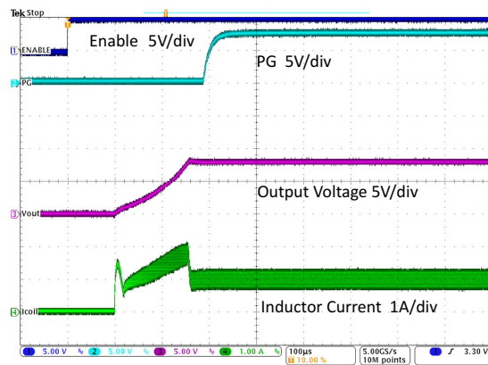
图 9-24. Startup After Enable
