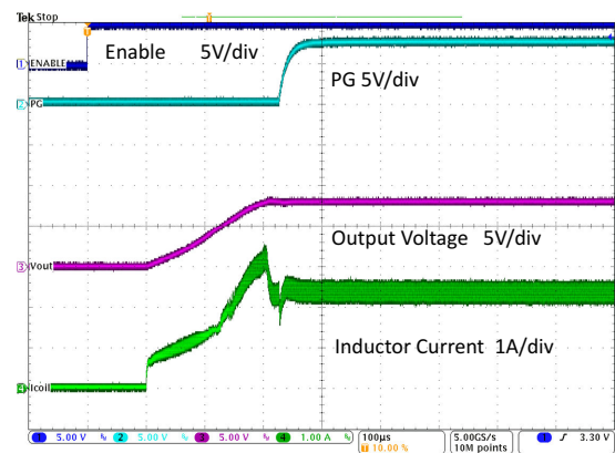
图 9-23. Startup After Enable
