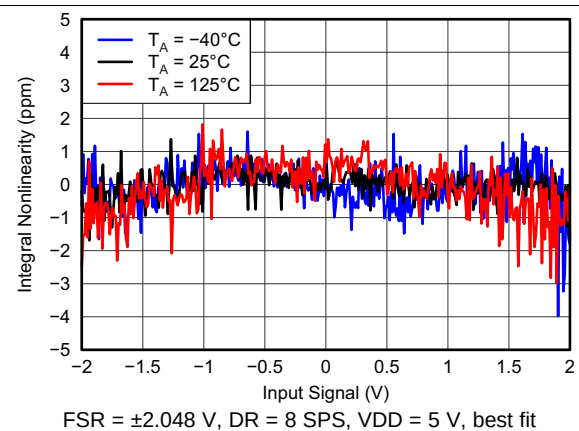
Figure 7. INL vs Input Signal
