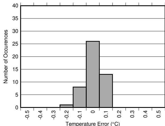
Figure 22. Temperature Sensor Error Histogram (VSSOP)
