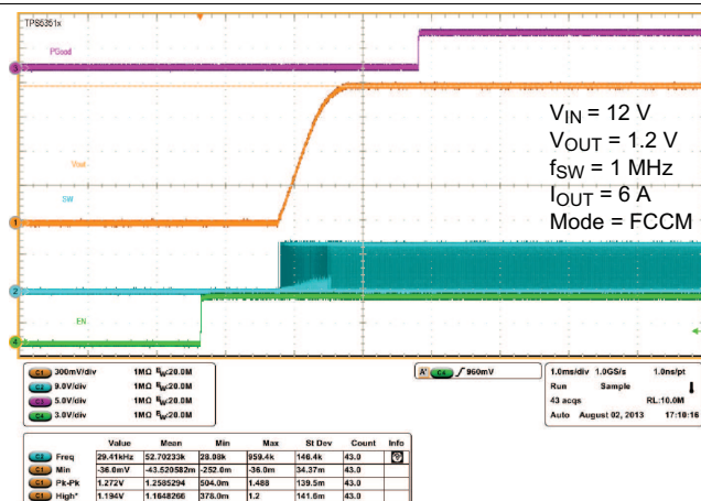
Figure 22. FCCM Start-Up
