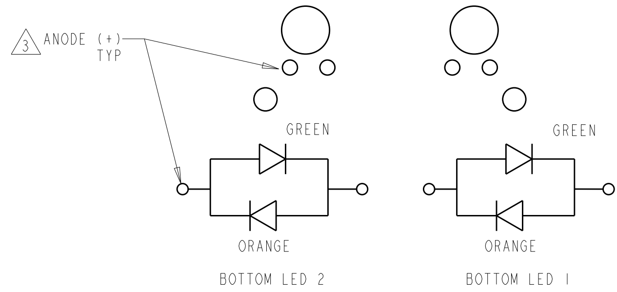
SCHEMATIC FOR 2-6368011-1 SCALE 4:1
