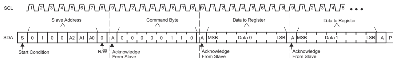
图 8-9. Write To Configuration Registers
