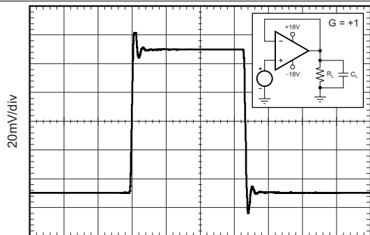
Time (1μs/div) G = +1 , R_L = 10k\Omega , C_L = 100pF
