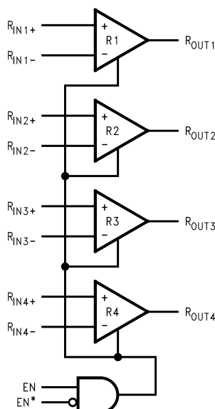
Functional Diagram
