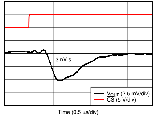
DAC code transition from midscale – 1 to midscale LSB, REF-DIV = 0 and BUFF-GAIN = 0
