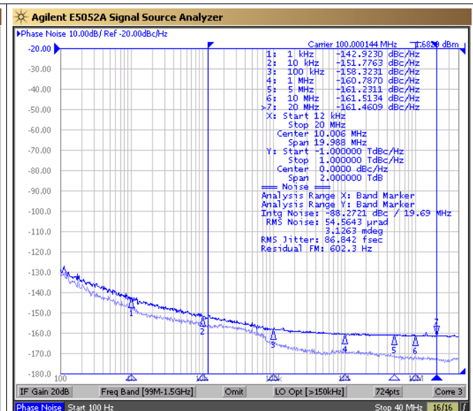
Figure 12. CDCLVC11xx Output Phase Noise 86 fs (12 kHz to 20 MHz)
