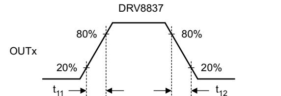
图 6-2. Input and Output Timing for DRV8837
