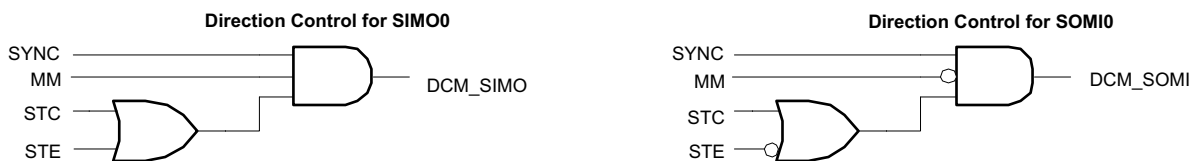
Figure 6-10. Direction Control for SMO0 and SOM0
