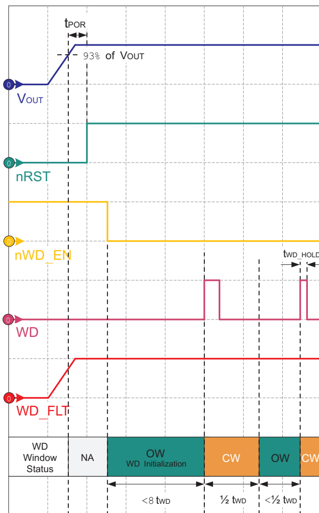
Figure 23. Power Up, Initialization, and Normal Operation for TPS7A63-Q1
