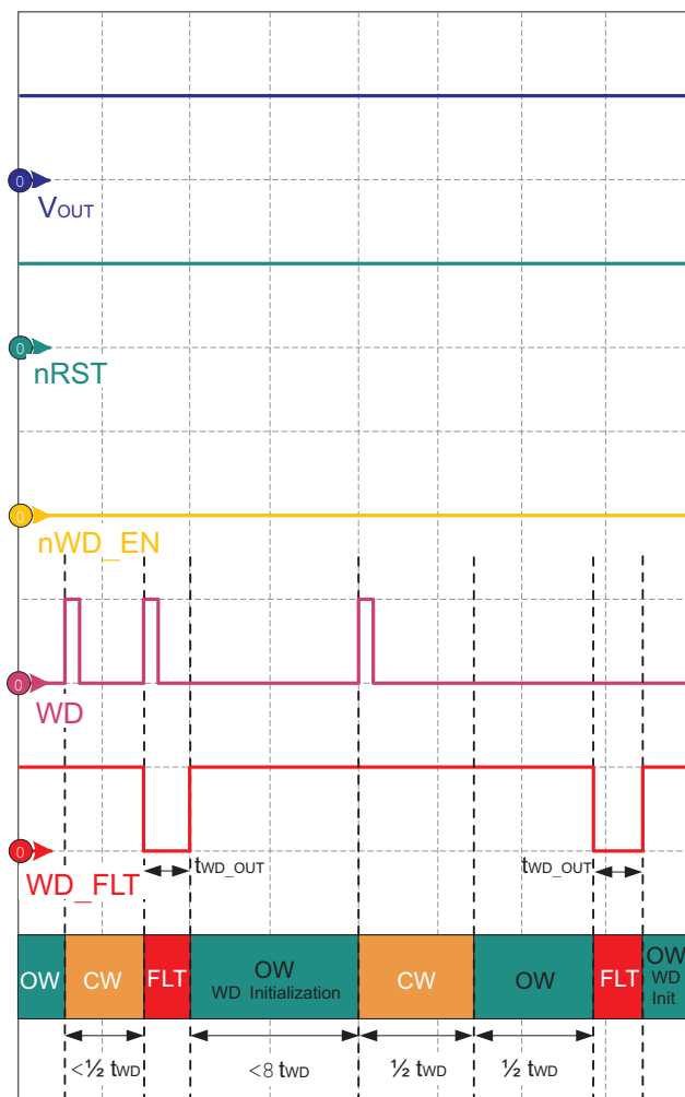
Figure 25. Watchdog Service Fault Conditions for TPS7A63-Q1
