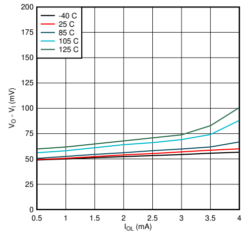
图 6-4. V_{OS} vs I_{OL} ( V_{CC} = 3.3 V, V_I = 0 V)
