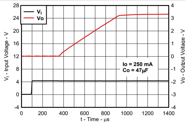
图 7-12. TPS76633 Output Voltage vs Time (New Chip)
