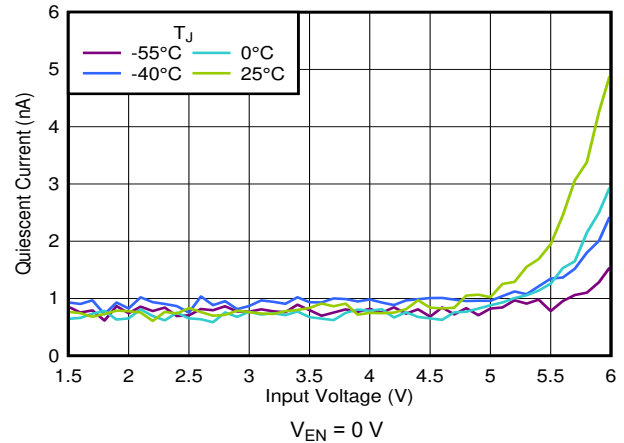
图 6-10. I_{SHDN} vs V_{IN} and Temperature
