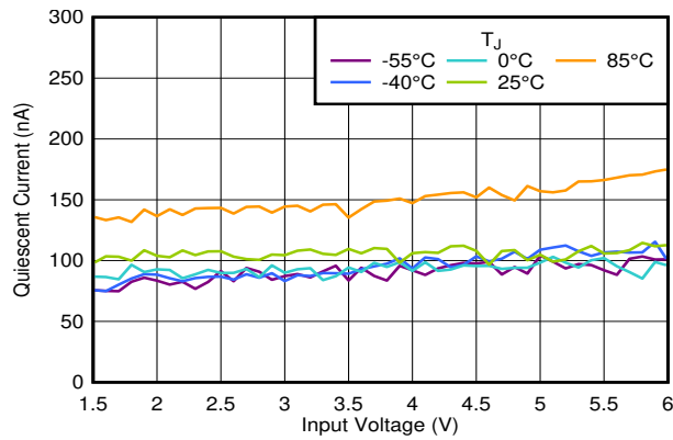
图 6-1. I_Q vs V_{IN} and Temperature
