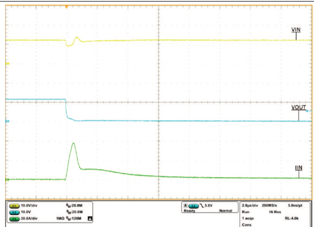
图 35. Output Hot Short to GND Response (Zoomed In)
