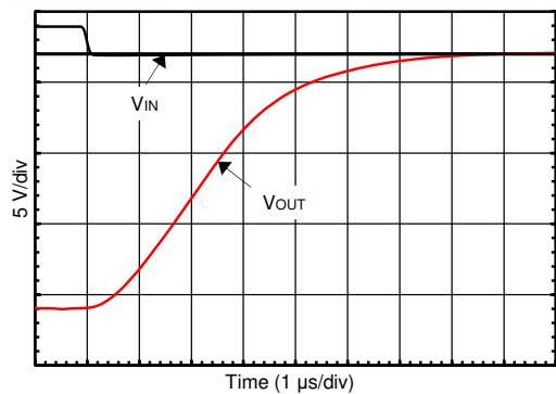
图 7-27. Positive Overload Recovery
