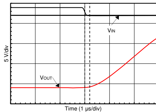
图 7-28. Positive Overload Recovery (Zoomed In)
