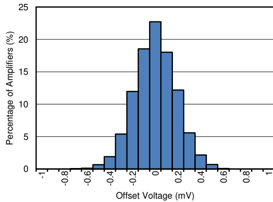
图 7-1. Offset Voltage Production Distribution
