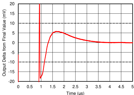
图 7-37. Large-Signal Settling Time (10-V Positive Step)
