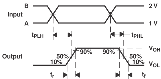
图 7-1. Switching Test Circuit and Voltage Waveforms
