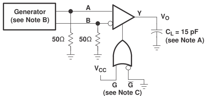
图 7-1. Switching Test Circuit and Voltage Waveforms
