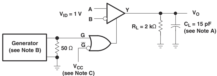
图 7-1. Switching Test Circuit and Voltage Waveforms
