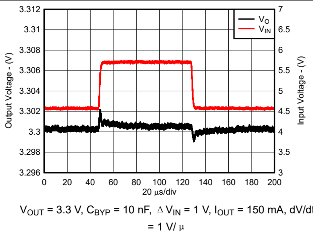
图 8-12. Line Transient Response for New Chip
