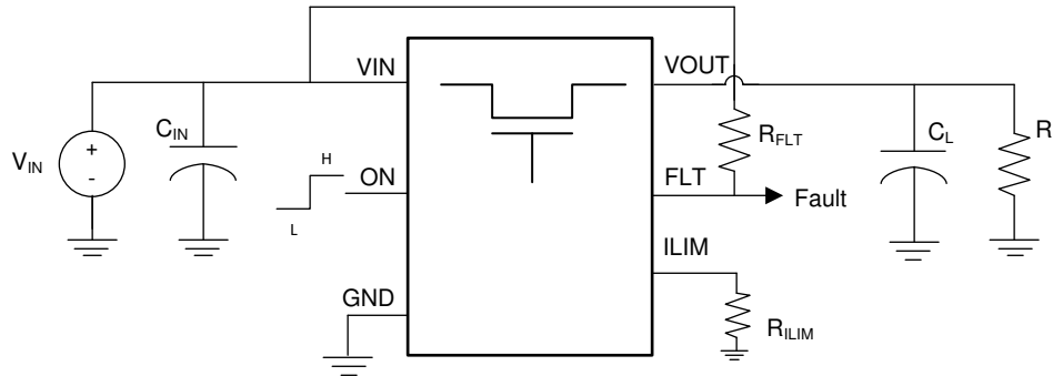
图 10-1. Typical Application
