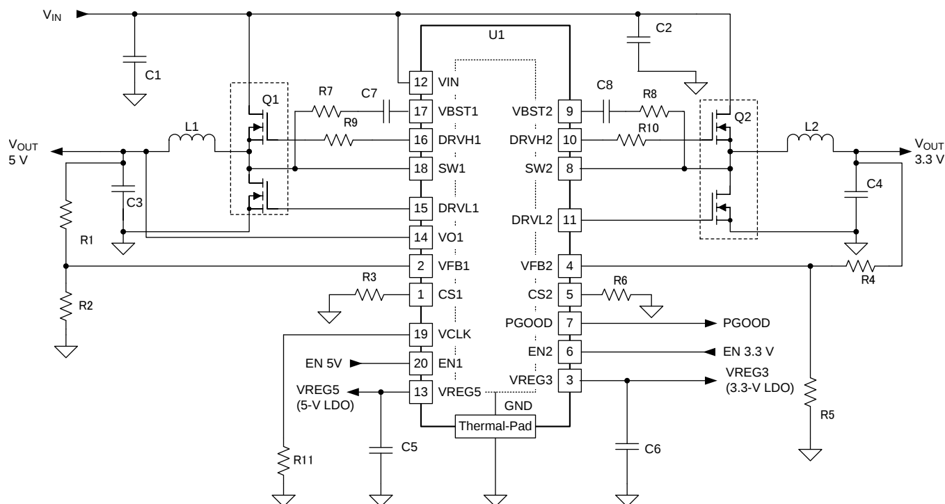
Figure 6. Application Schematic
