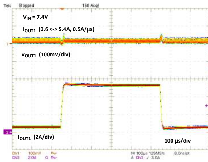
Figure 25. Load Transient
