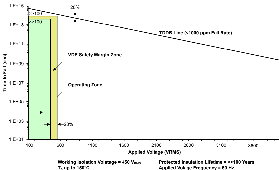
图 9-8. Insulation Lifetime Projection Data for 8-D Package
