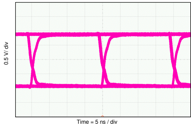
图 9-6. Eye Diagram at 50 Mbps PRBS 2^{16} - 1 , 1.8 V and 25°C
