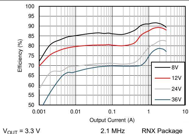
图 9-18. Efficiency
