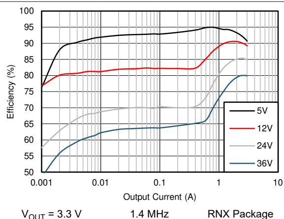
图 9-16. Efficiency
