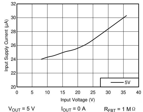
图 9-20. Input Supply Current
