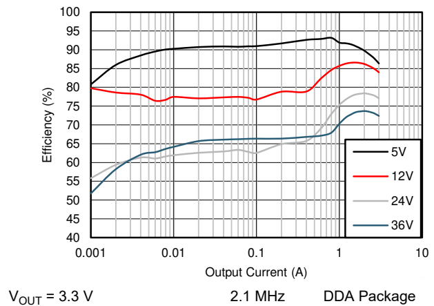
图 9-12. Efficiency
