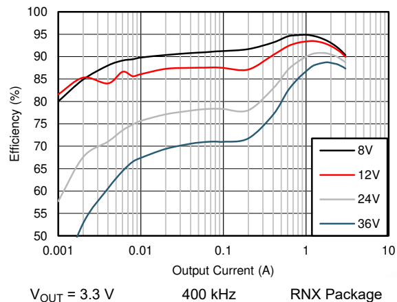
图 9-14. Efficiency
